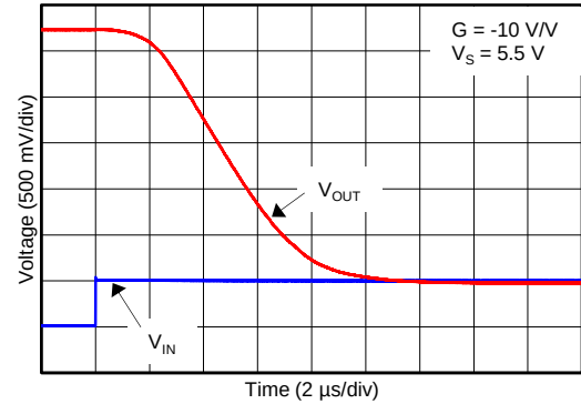
Figure 26. 正过载恢复
