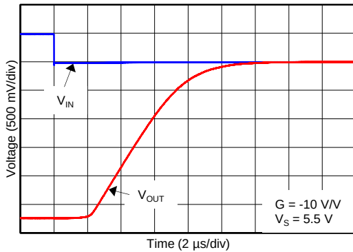
Figure 27. 负过载恢复
