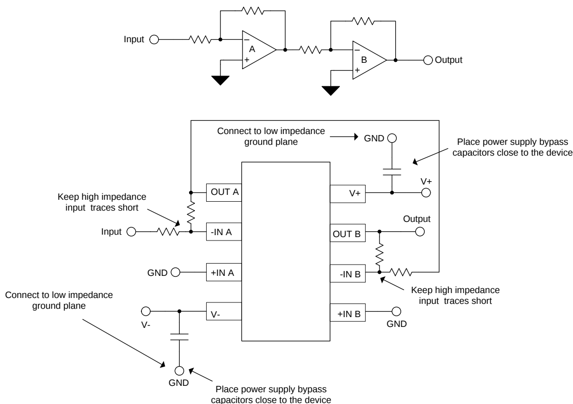
Figure 48. Layout Example
