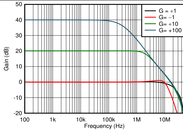
图 19. Closed-Loop Gain vs Frequency
