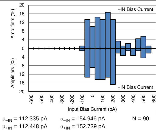
图 3. Input Bias Current Production Distribution
