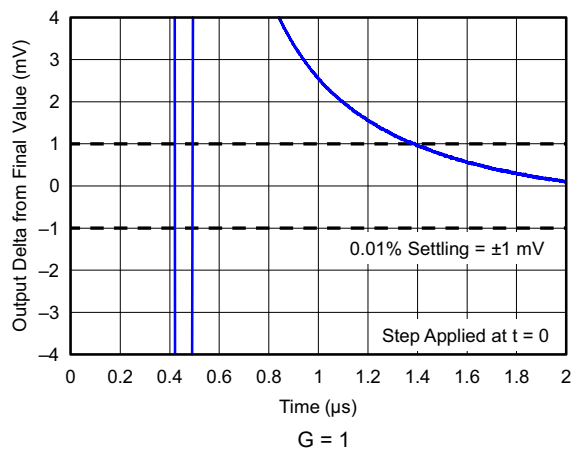
图 6-40. Settling Time (10-V Negative Step)
