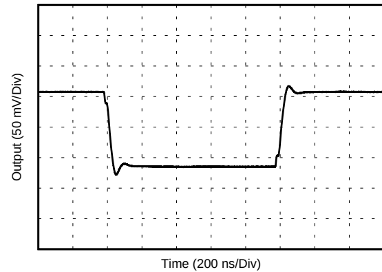
Figure 32. Small-Signal Step Response
