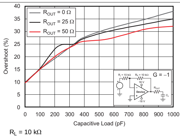
图 11. Small-Signal Overshoot vs Capacitive Load (100-mV Output Step)
