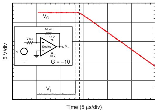
图 13. Positive Overload Recovery
