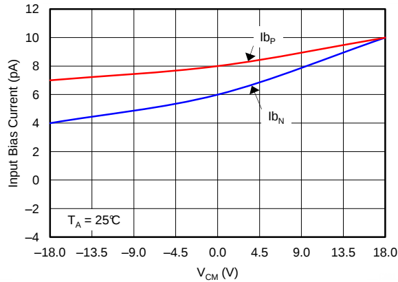
图 7. Input Bias Current vs Common-Mode Voltage
