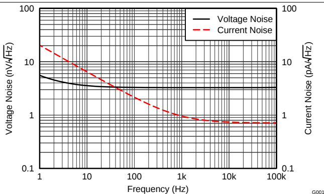
Figure 1. Input Voltage Noise Density and Input Current Noise Density vs Frequency
