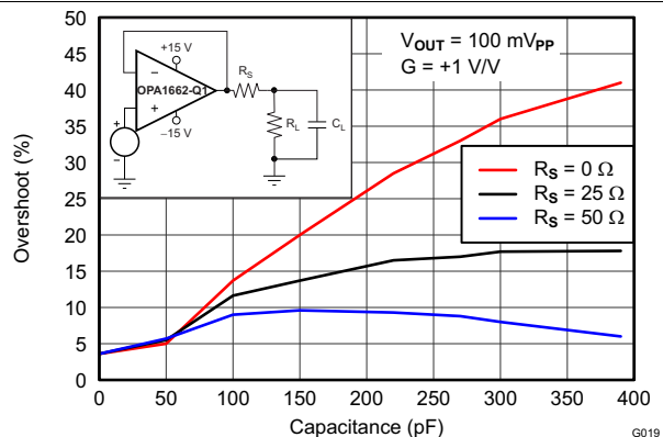
Figure 25. Small-Signal Overshoot vs Capacitive Load
