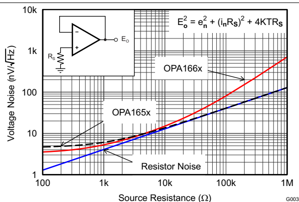
Figure 3. Voltage Noise vs Source Resistance
