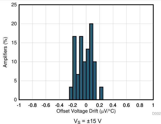
图 6-15. Input Offset Voltage Drift Histogram
