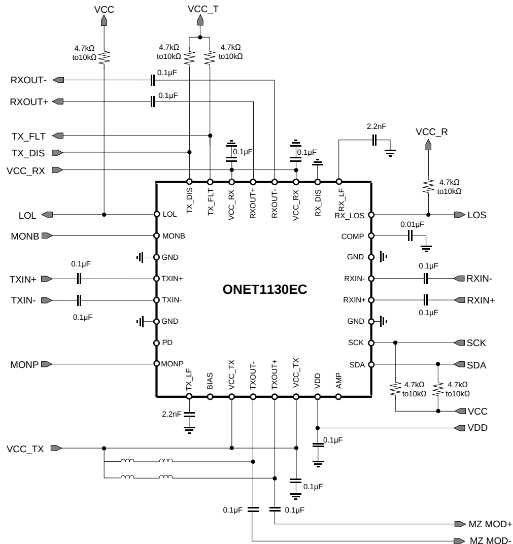
图 68. Typical Application Circuit in Differential Mode
