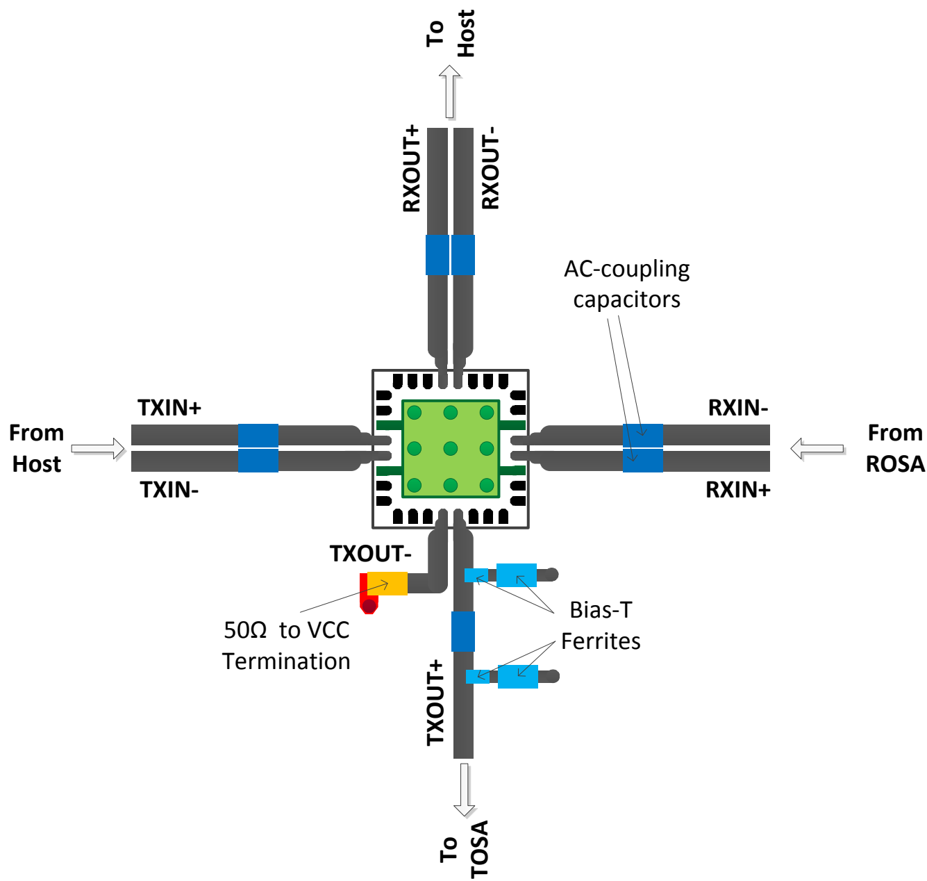
图 73. Board Layout
