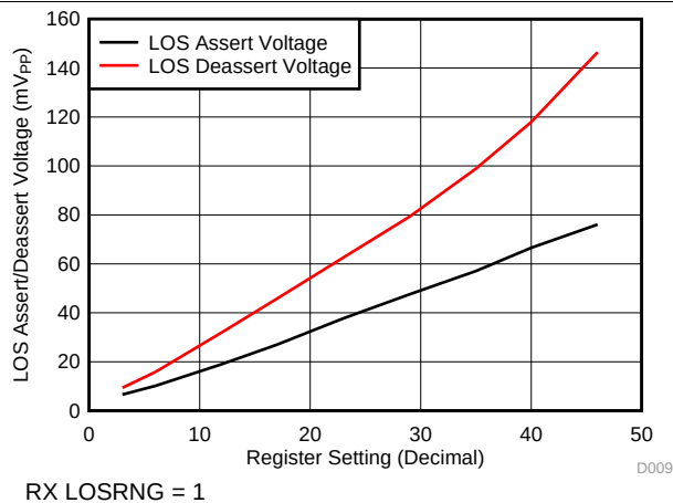
Figure 31. LOS Assert / Deassert Voltage vs Register 7 Setting
