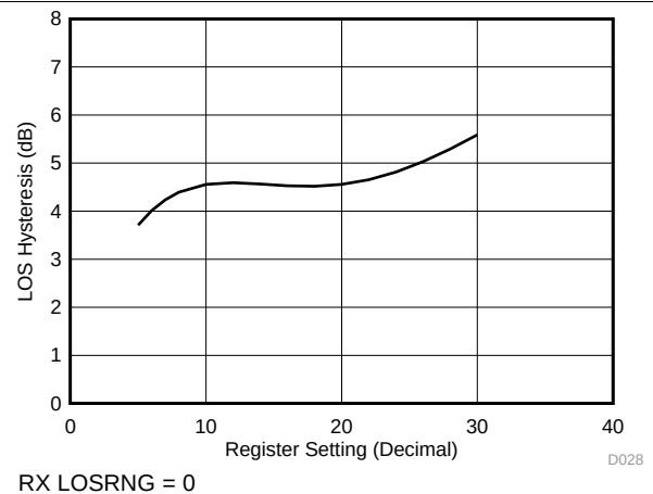
Figure 32. LOS Hysteresis vs Register 7 Setting
