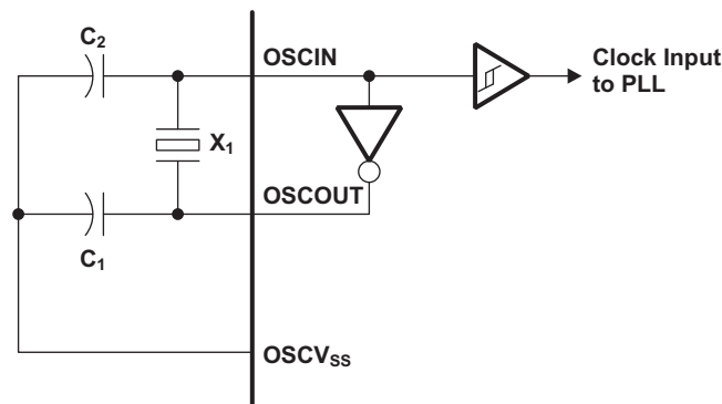
Figure 5-7. On-Chip 1.2V Oscillator
