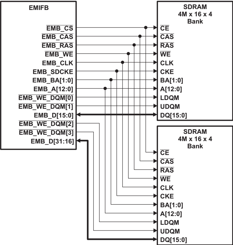
Figure 5-24. EMIFB to Dual 4M × 16 × 4 bank SDRAM Interface
