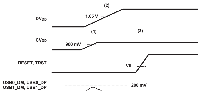
Figure 5-4. Power Sequence
