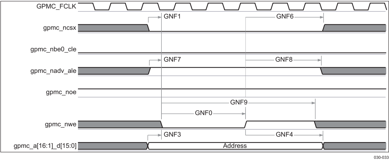
Figure 6-14. GPMC/NAND Flash – Address Latch Cycle Timing
