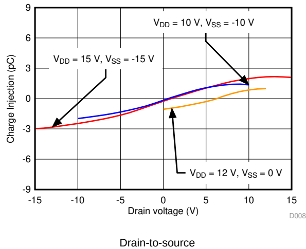
图 13. Charge Injection vs Drain Voltage
