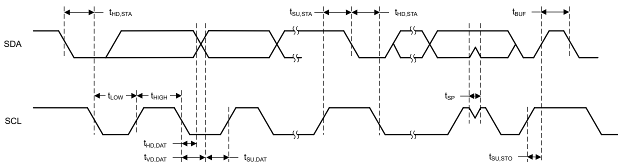
图 7-3. I2C Timing Diagram
