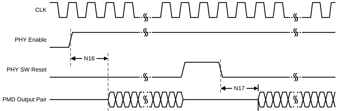
图 5-34. Reset Timing
