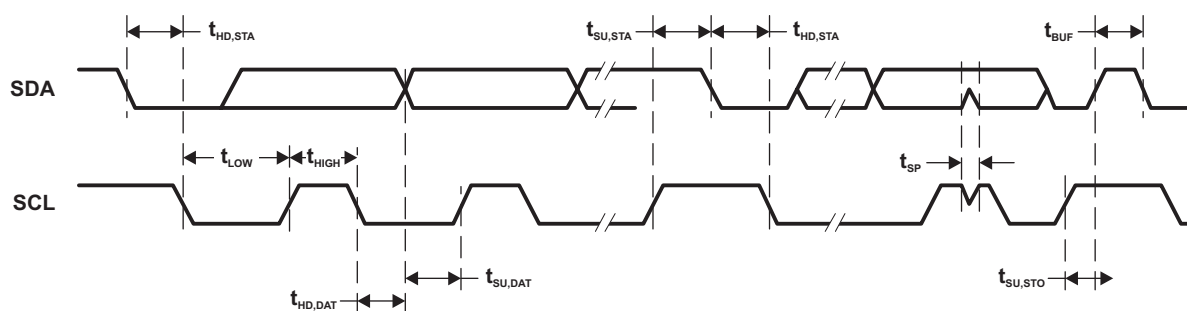
Figure 20. I2C Mode Timing
