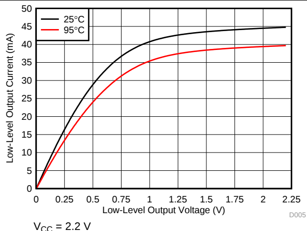
Figure 4-9. Typical Low-Level Output Current vs Low-Level Output Voltage
