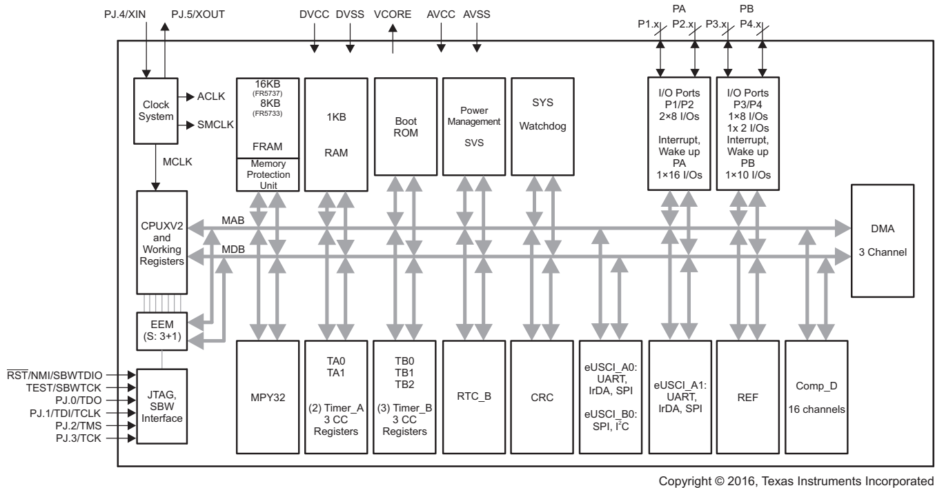
图 6-2. Functional Block Diagram – RHA Package – MSP430FR5733, MSP430FR5737
