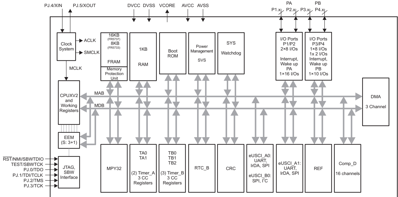
图 6-2. Functional Block Diagram – RHA Package – MSP430FR5733, MSP430FR5737
