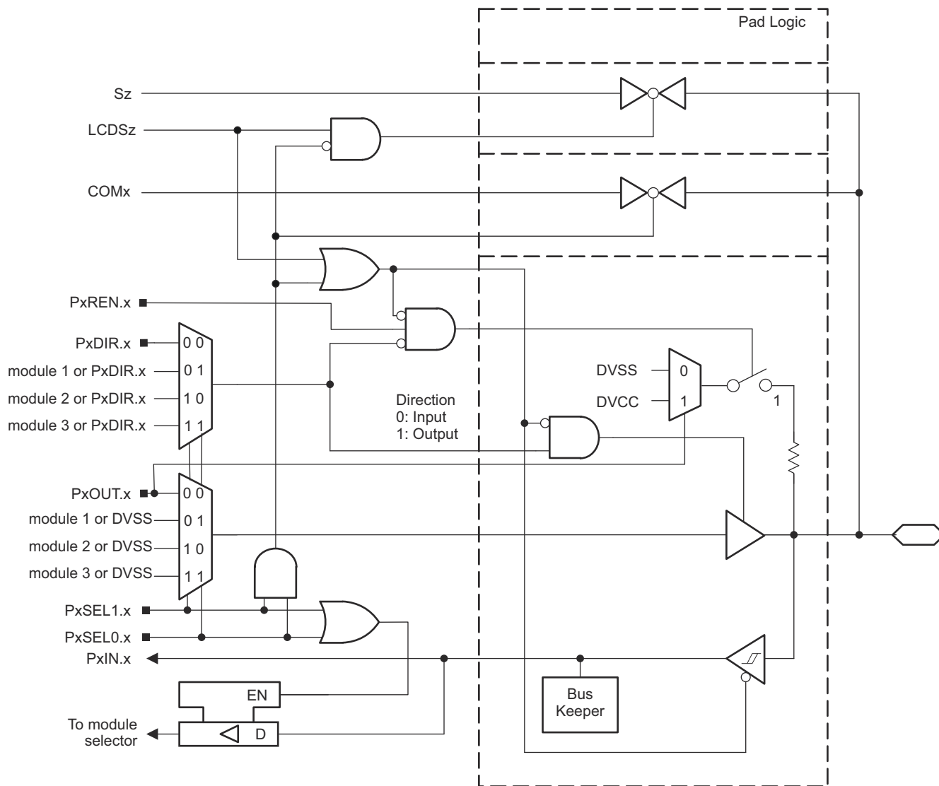
图 9-14. Port P3 (P3.4 to P3.5) Diagram
