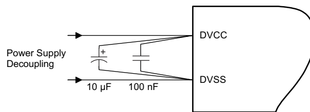
图 10-1. Power Supply Decoupling
