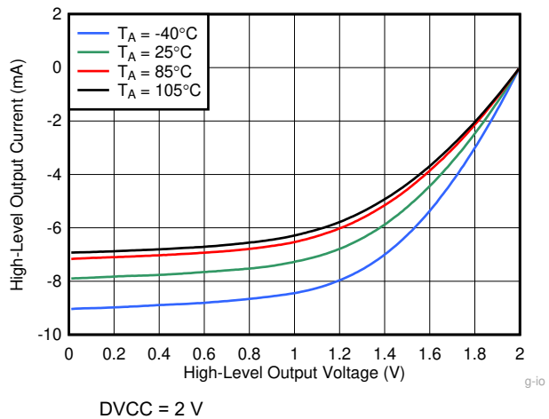
图 8-10. Typical High-Level Output Current vs High-Level Output Voltage
