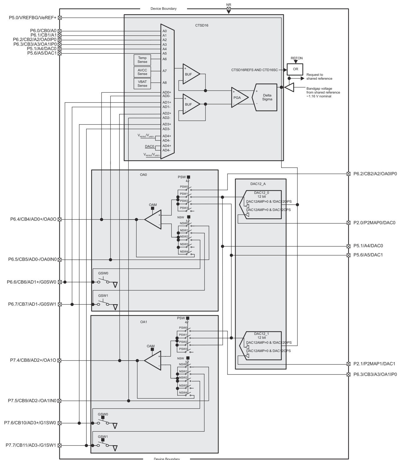
图 9-2. Signal Chain
