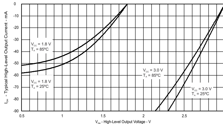
图 8-31. Ports PU.0, PU.1 Typical High-Level Output Characteristics
