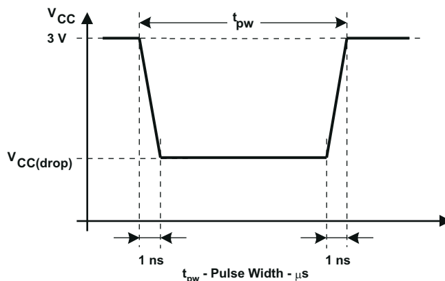
图 8-11. V_{CC(drop)} Level with a Square Voltage Drop to Generate a POR or BOR Signal
