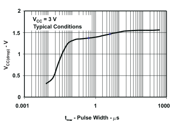
图 8-11. V_{CC(drop)} Level with a Square Voltage Drop to Generate a POR or BOR Signal
