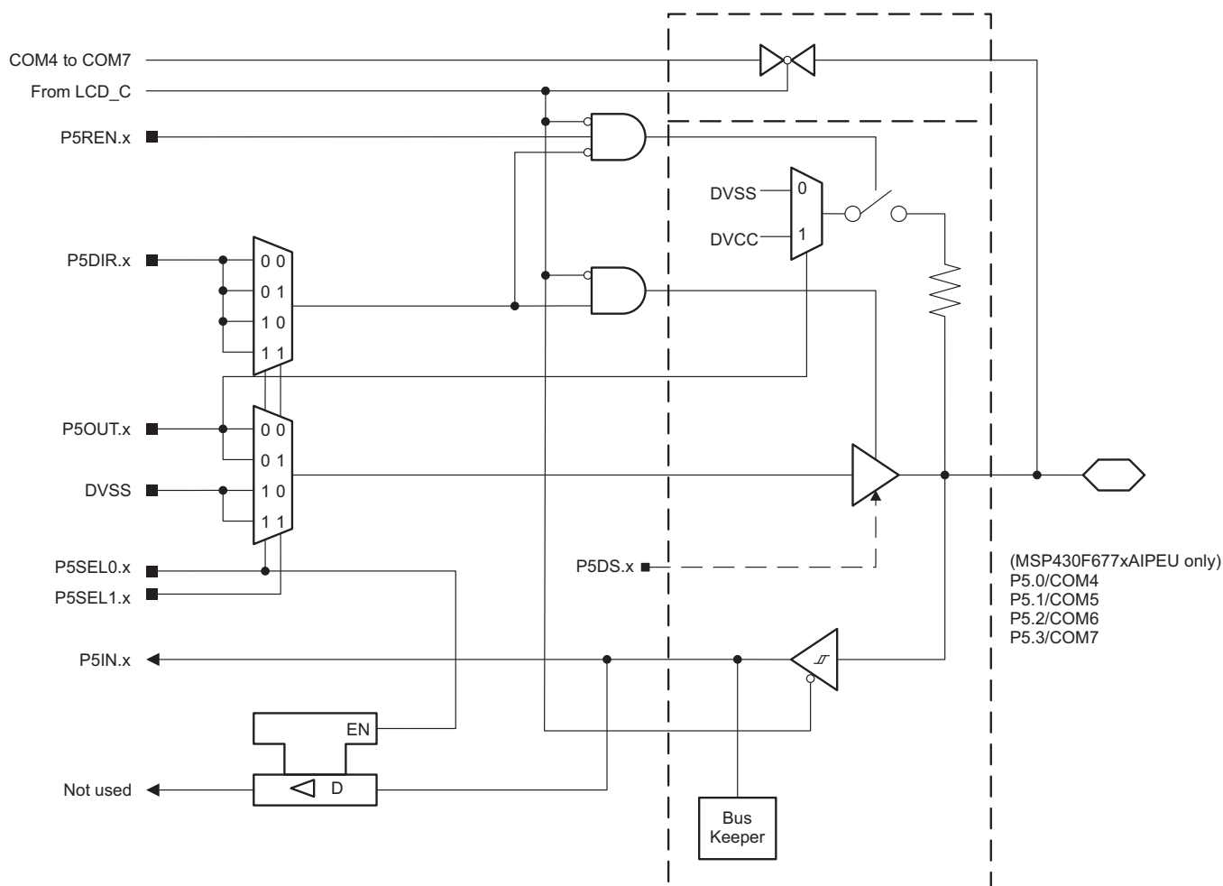
Figure 6-19. Port P5 (P5.0 to P5.3) Diagram (PEU Package Only)
