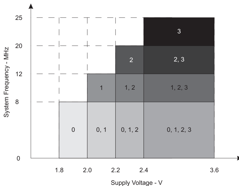
Figure 3. Frequency vs Supply Voltage
