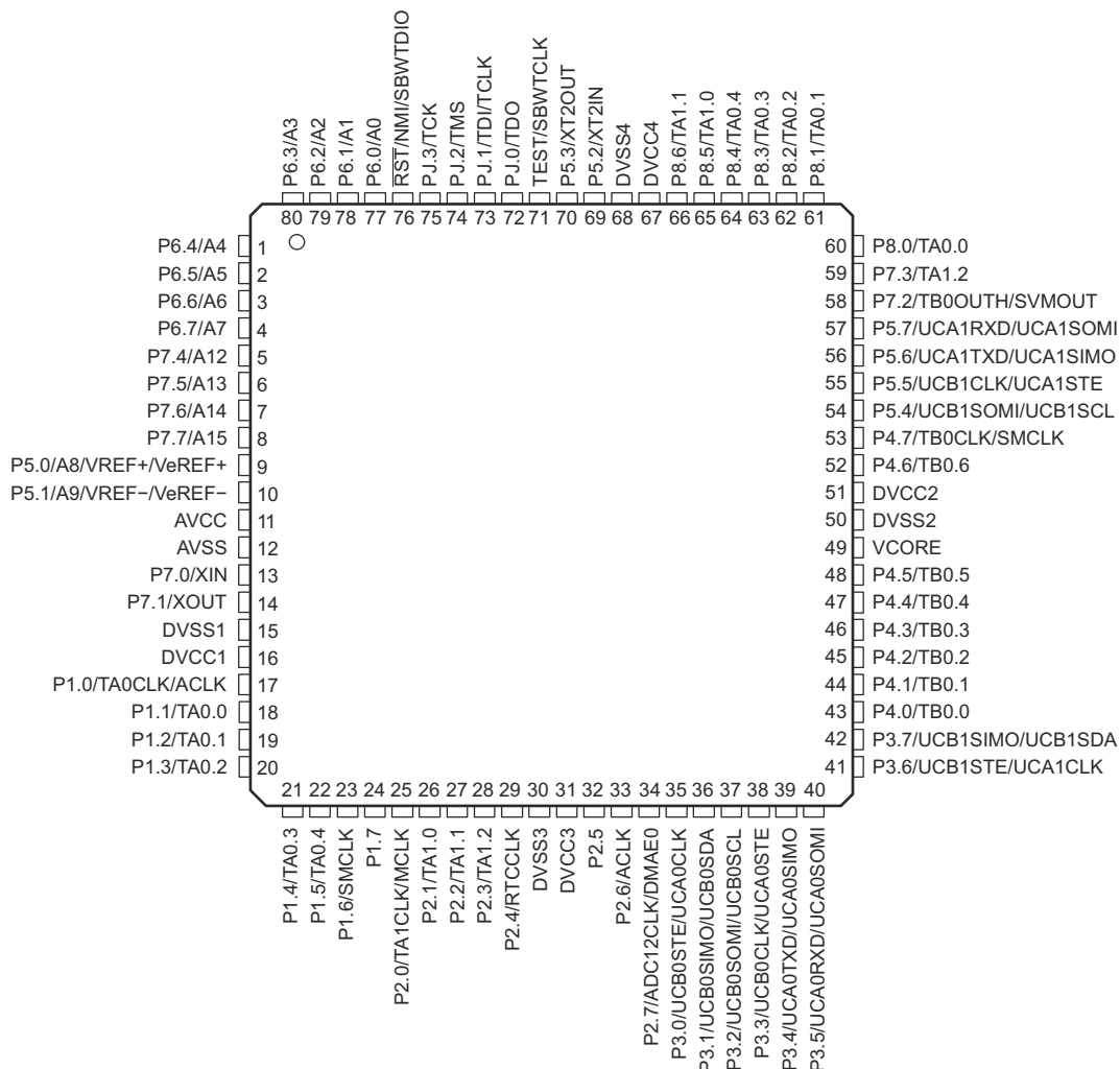
图 7-2. 80-Pin PN Package (Top View) - MSP430F5437AIPN, MSP430F5435AIPN, MSP430F5418AIPN
