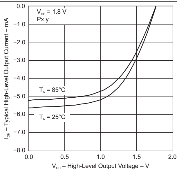
图 5-6. Typical High-Level Output Current vs High-Level Output Voltage
