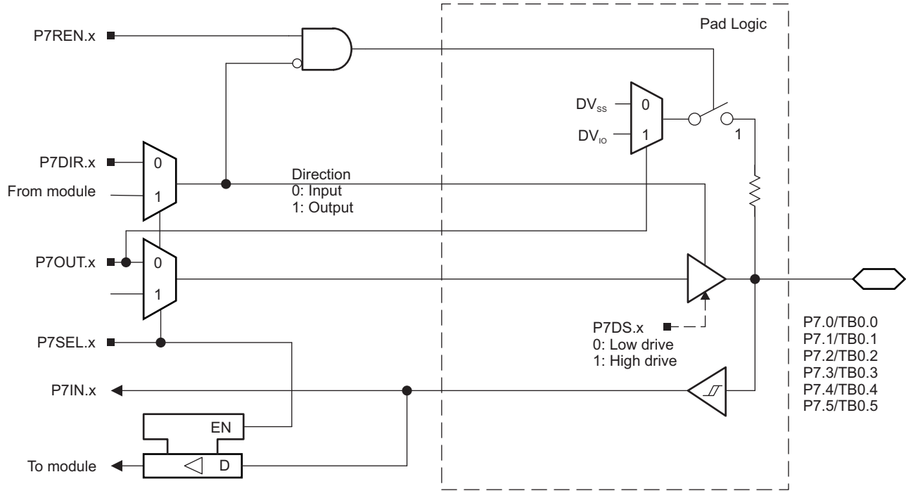
图 6-12. Port P7 (P7.0 to P7.5) Diagram
