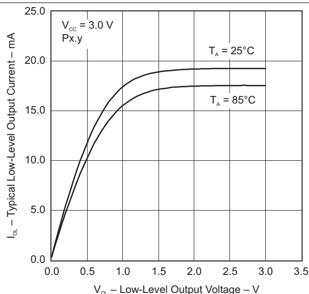
图 5-3. Typical Low-Level Output Current vs Low-Level Output Voltage
