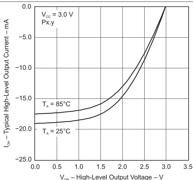
图 5-5. Typical High-Level Output Current vs High-Level Output Voltage
