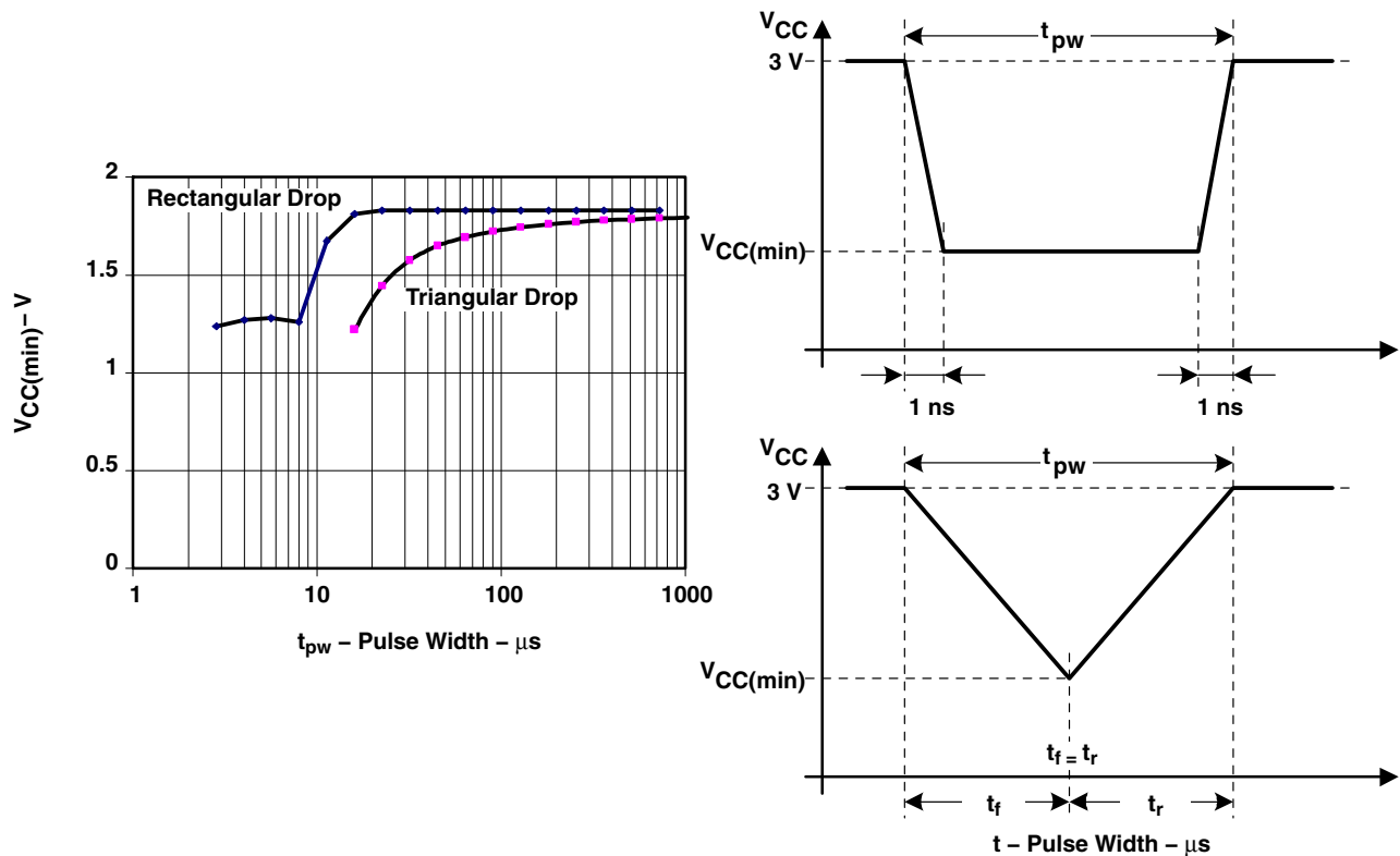
Figure 12. V_{CC(min)} With a Square Voltage Drop and a Triangle Voltage Drop to Generate an SSV Signal
