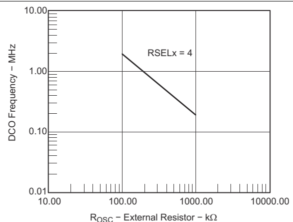
图 8-20. DCO Frequency vs R_{OSC} (V CC = 3 V, T A = 25°C)
