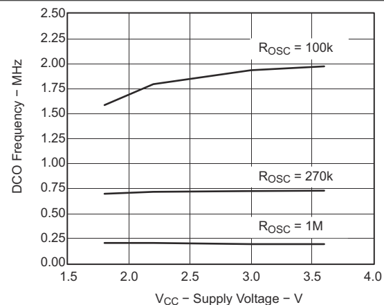
图 8-22. DCO Frequency vs Supply Voltage (T A = 25°C)
