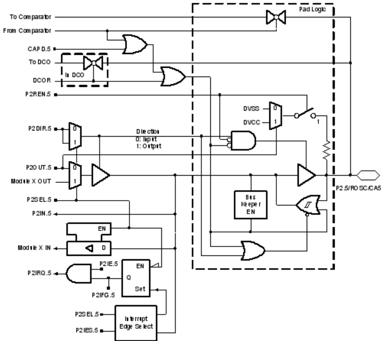
Port P2.5 pin functions
