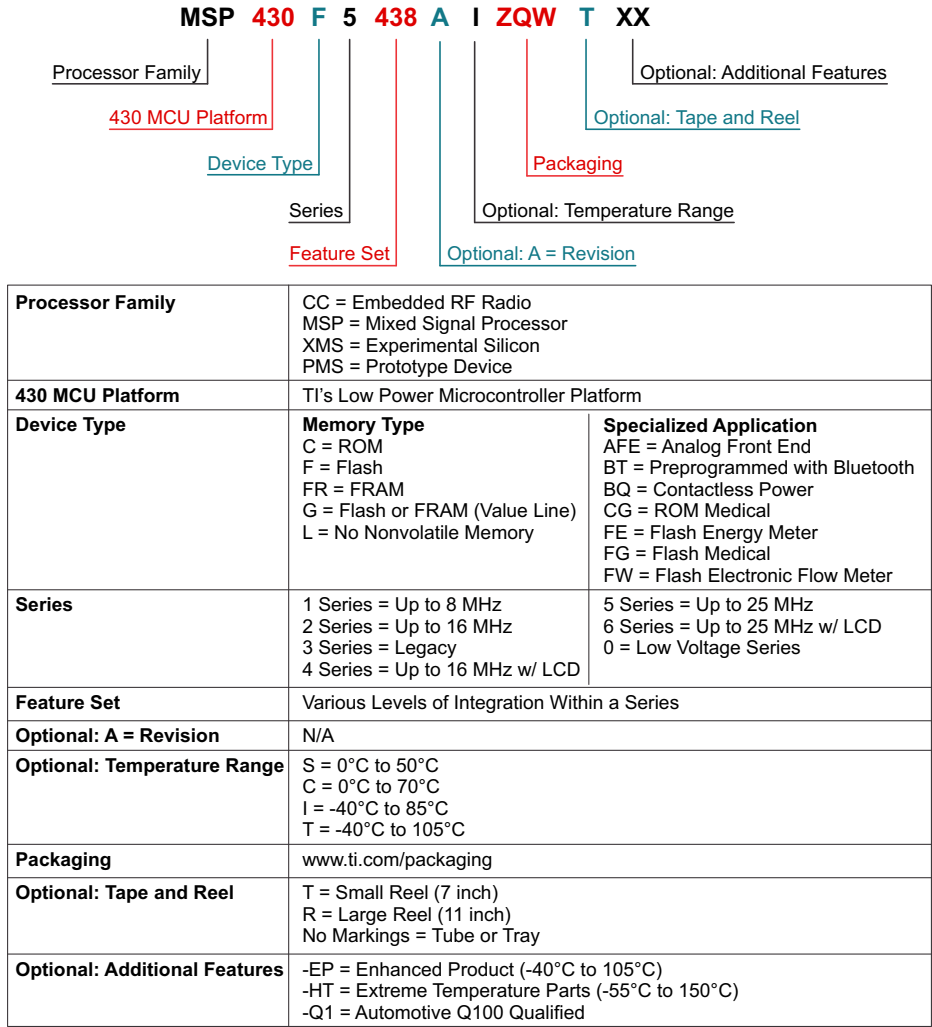
Figure 27. Device Nomenclature
