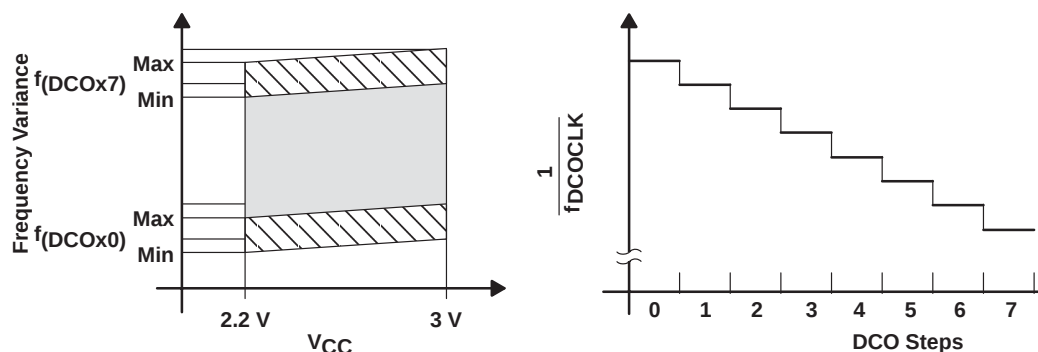
Figure 4. DCO Characteristics
