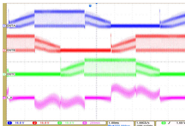
图 9-11. Driver PWM Operation
