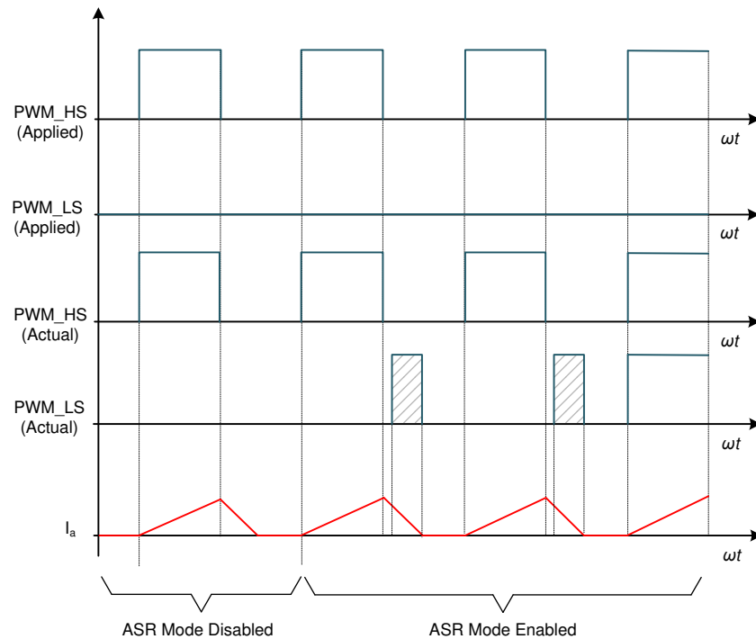
图 8-32. ASR in PWM Mode
