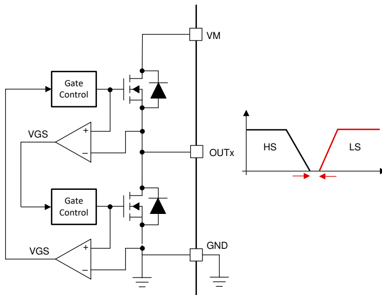
图 8-18. Cross Conduction Protection
