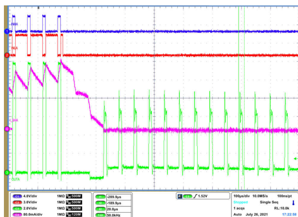
图 9-14. Driver PWM with Active Demagnetization (ASR and AAR)
