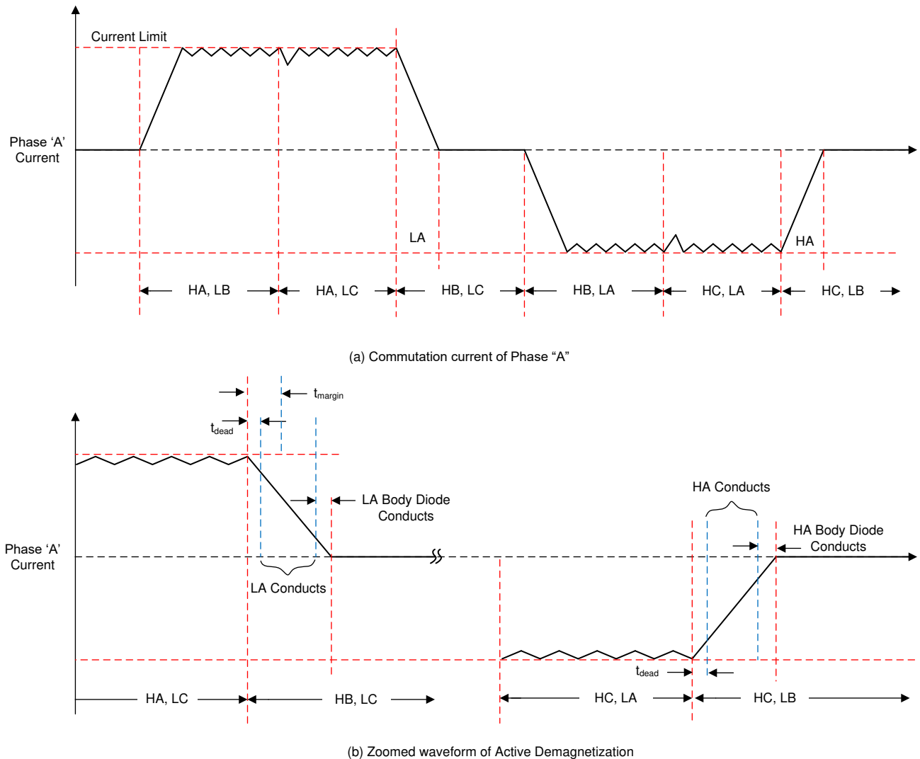
图 8-31. Current Waveforms for ASR in BLDC Motor Commutation
