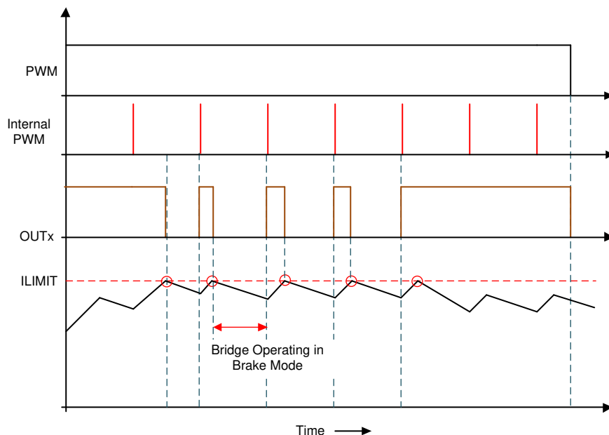
图 8-38. Cycle-by-Cycle Current-Limit Operation with 100% PWM Duty Cycle
