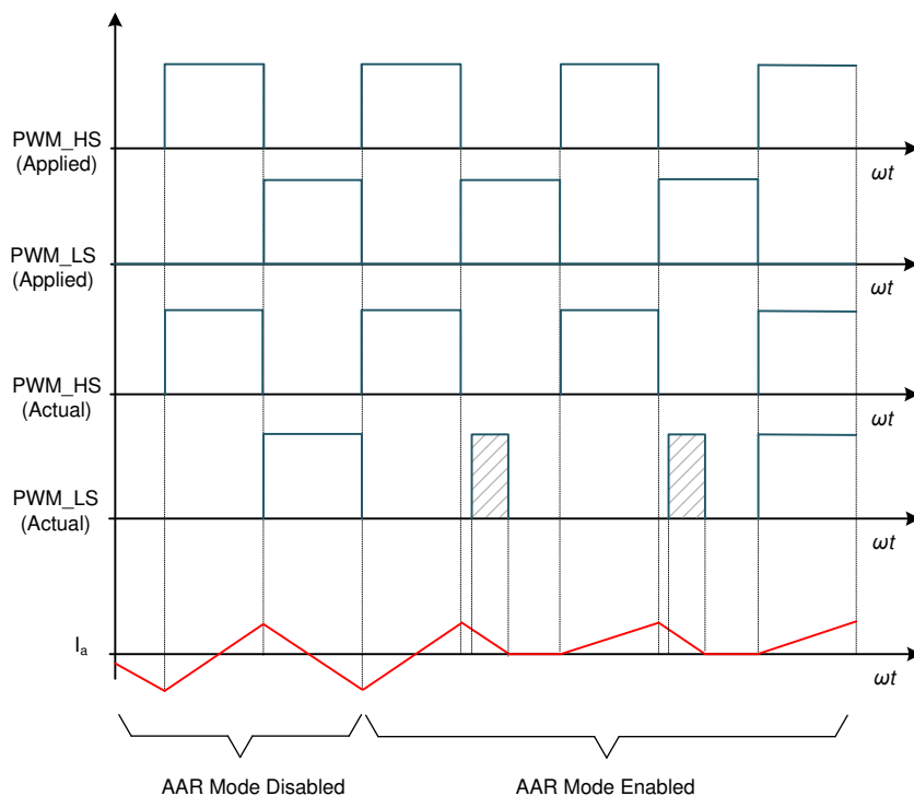
图 8-33. AAR in PWM Mode
