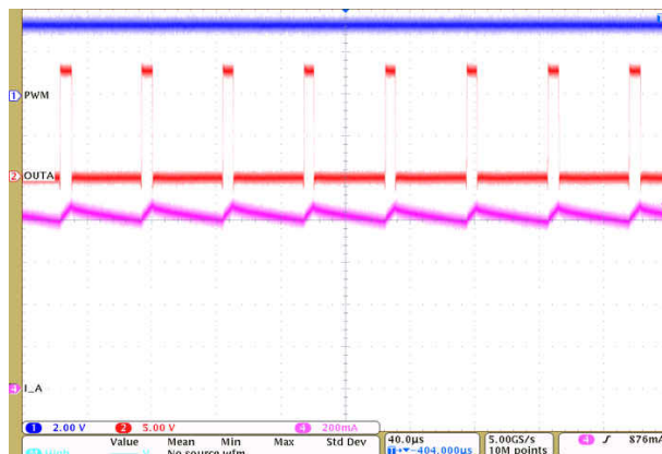
图 9-16. Driver 100% Operation with Current Chopping
