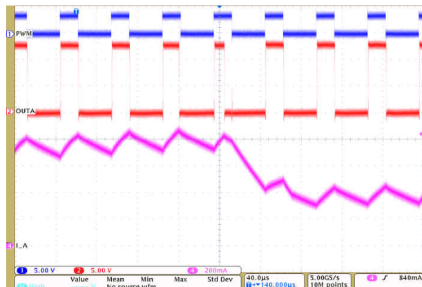
图 9-15. Driver PWM Operation with Current Limit
