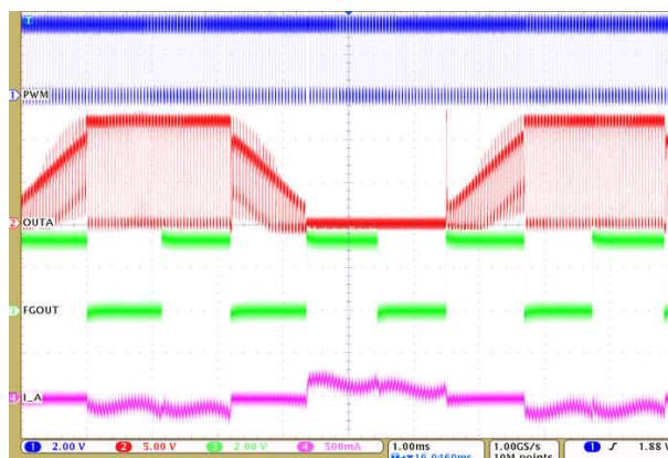
图 9-12. Driver PWM Operation with FGOUT
