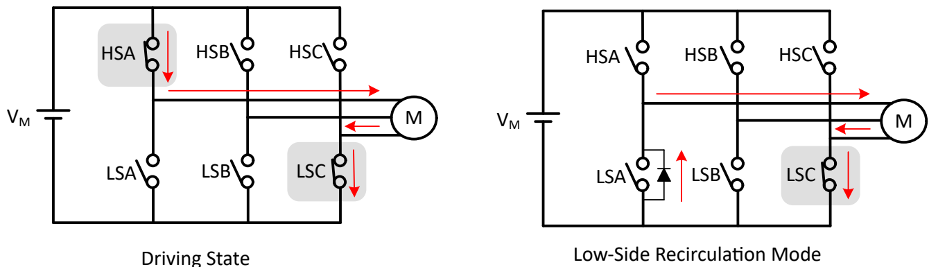
图 8-41. Low-Side Recirculation
