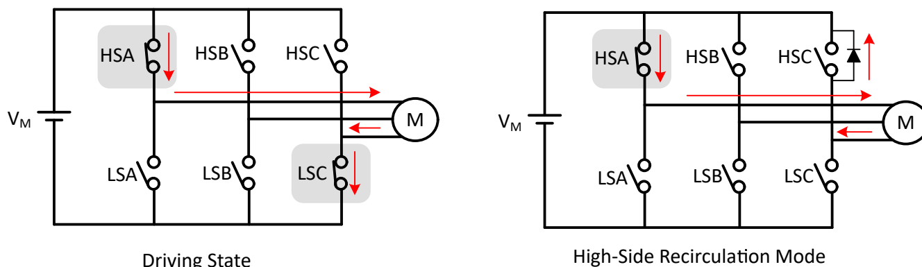
图 8-42. High-Side Recirculation
