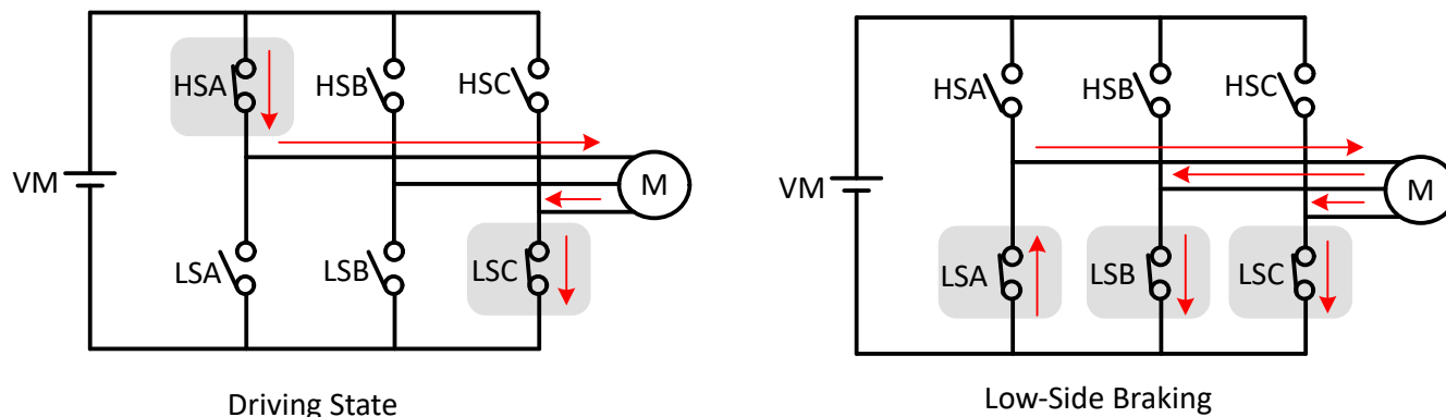
图 8-43. Low-Side Braking
