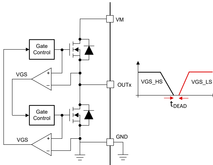
图 8-12. Cross Conduction Protection
