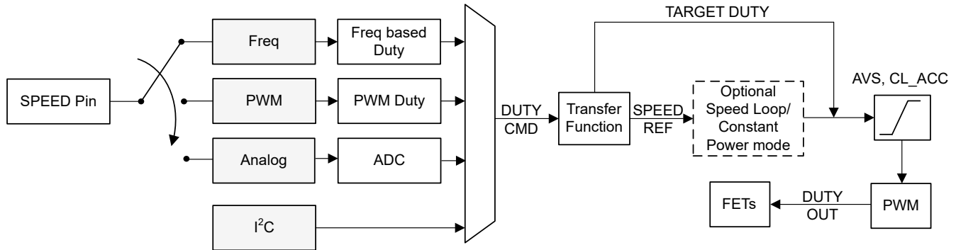
图 8-14. Multiplexing the Speed Command
