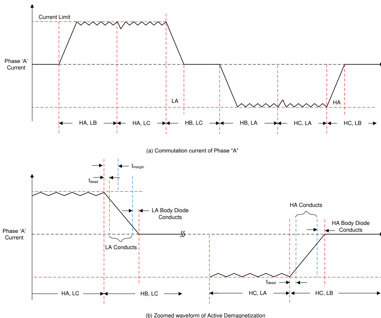
图 8-39. Current Waveforms with Active Demagnetization
