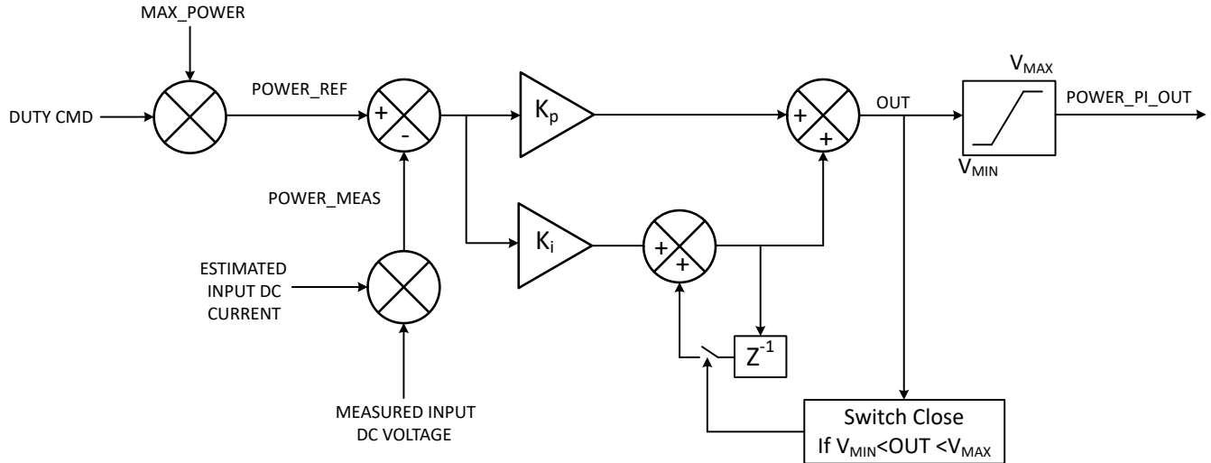
图 8-33. Power Regulation
