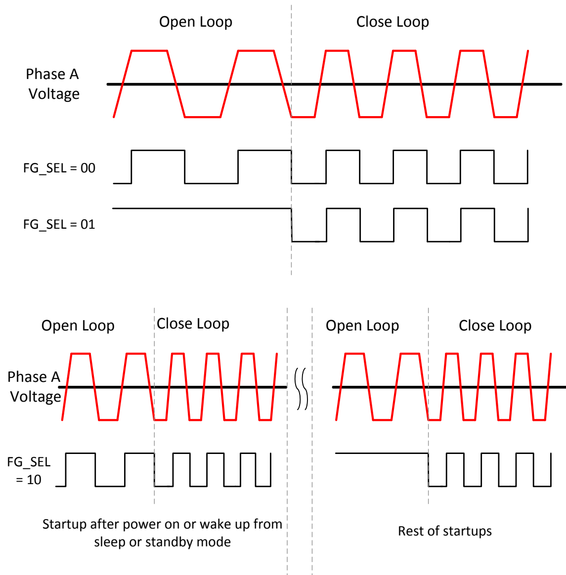
图 8-46. FG Behavior During Open Loop
