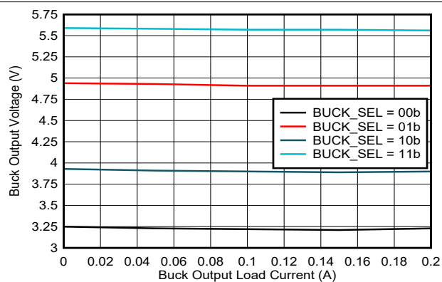
图 7-4. Buck regulator output voltage over load current
