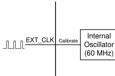
图 7-53. External Clock Reference
