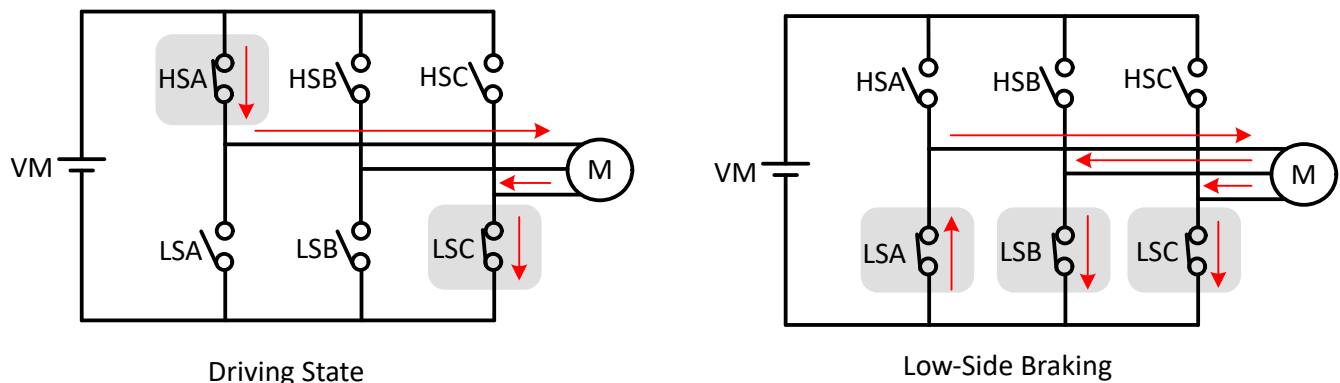
图 7-45. Low-Side Braking
