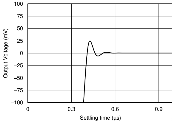
图 31. Large Signal Settling Time (Positive)
