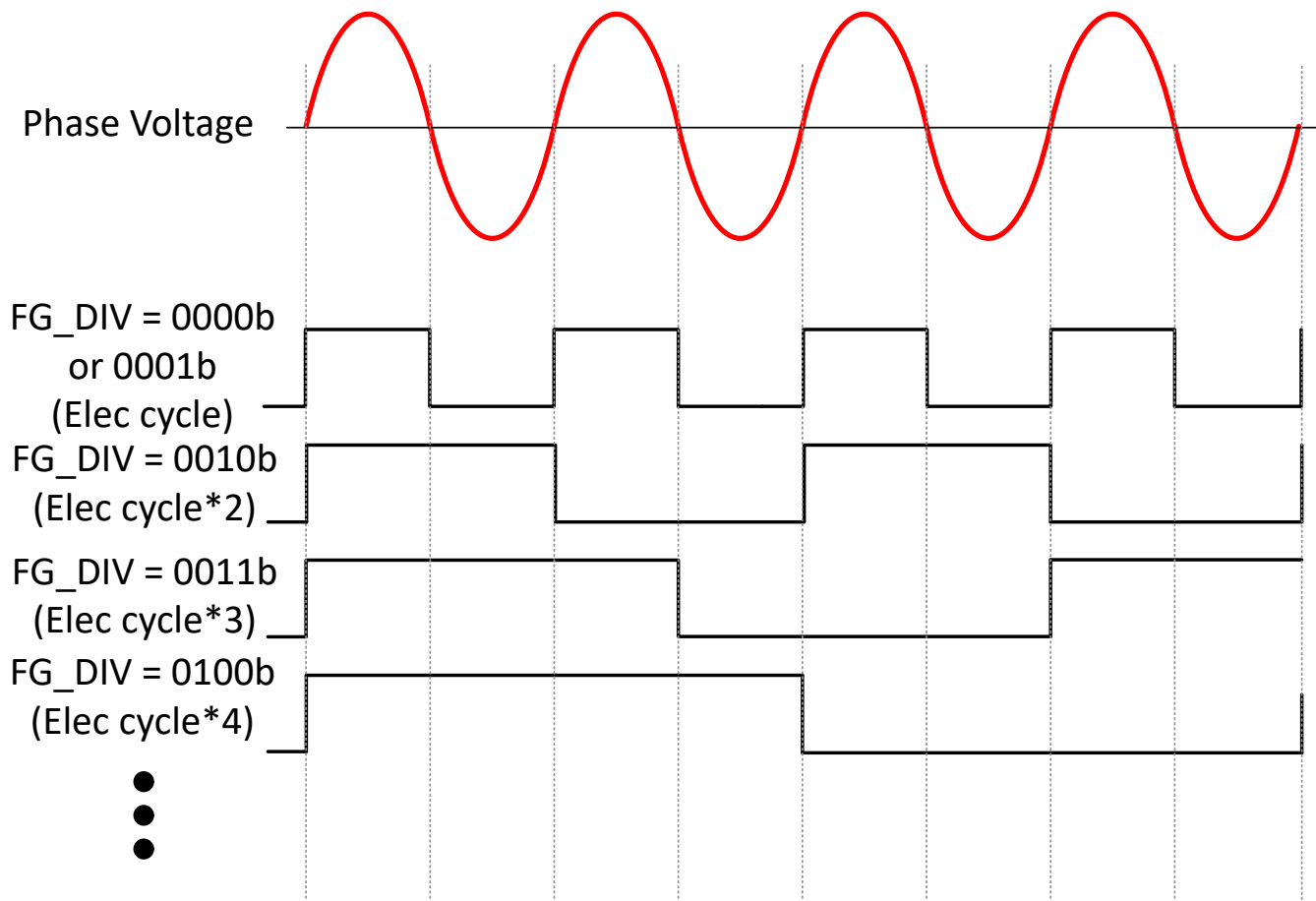
图 7-46. FG Frequency Divider
