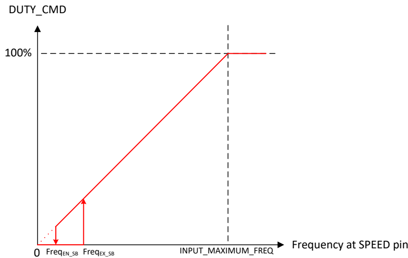
图 7-17. Frequency-Mode Motor Control
