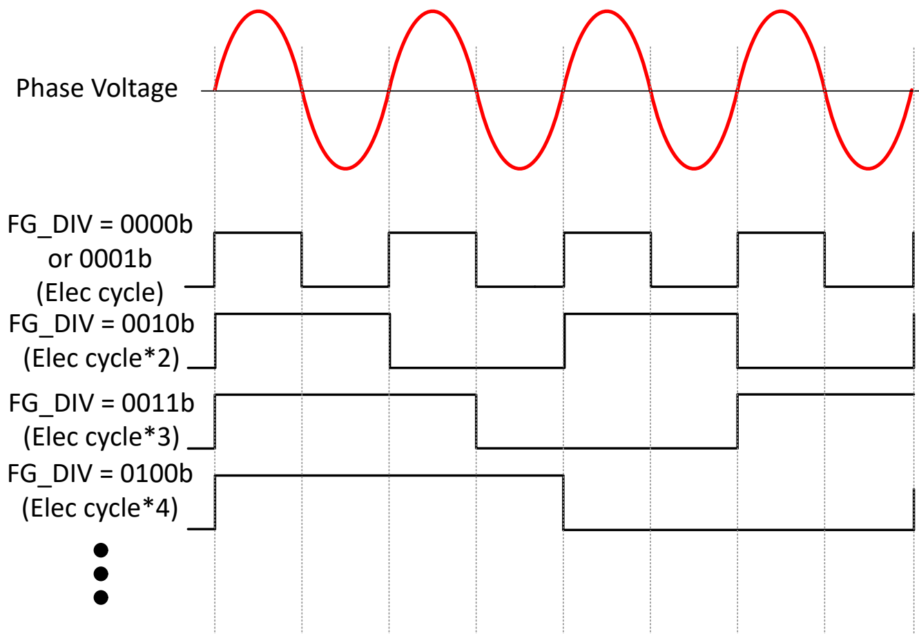
图 7-49. FG Frequency Divider
