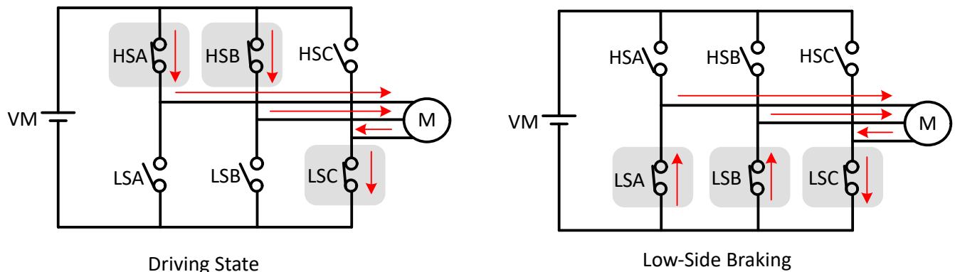
图 7-47. Low-Side Braking
