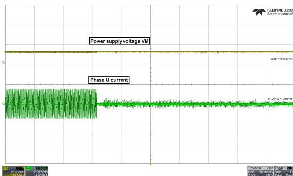
图 8-11. Power supply voltage and phase current waveform when AVS is enabled
