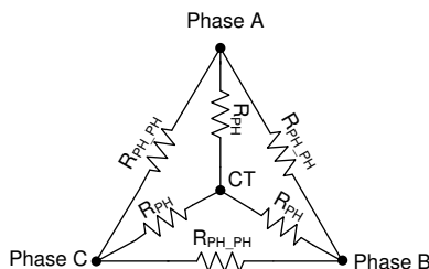
图 7-38. Motor Resistance
