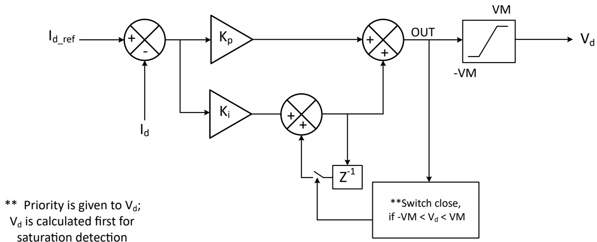
图 7-36. I_d Current PI Control
