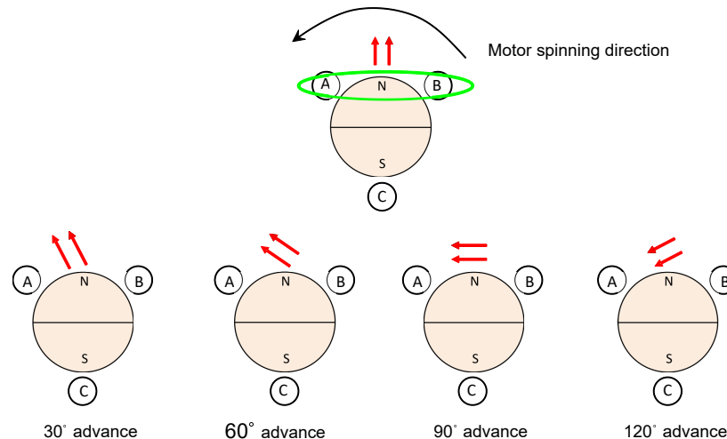
图 7-29. IPD Advance Angle
