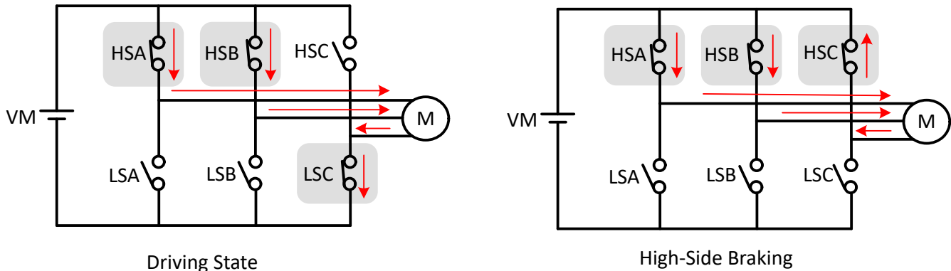
图 7-48. High-Side Braking
