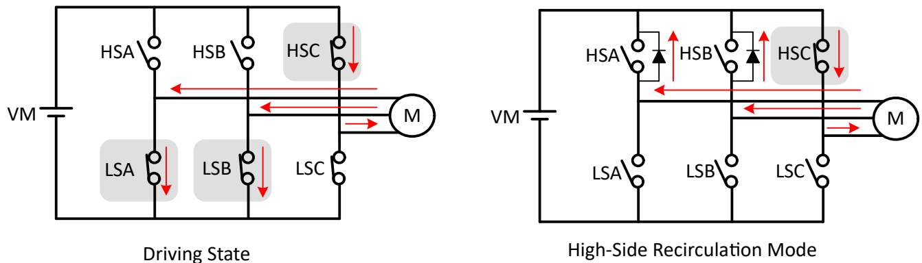
图 7-46. High-Side Recirculation
