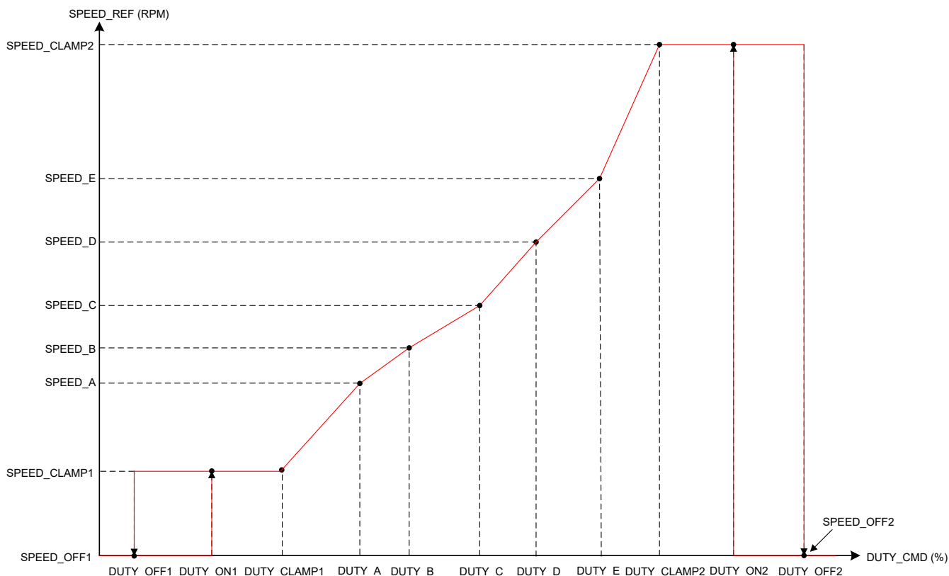
图 7-19. Linear Speed Profile
