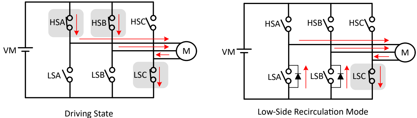
图 7-45. Low-Side Recirculation
