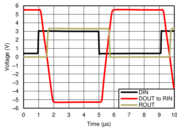
图 9-2. 250-kbps Driver to Receiver Loopback Timing Waveform, V_{CC} = 3.3 \text{ V}
