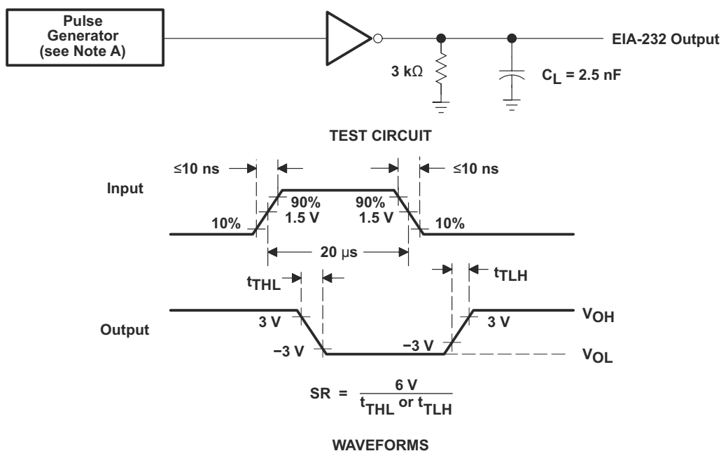
图 6-2. Driver Test Circuit and Waveforms for t_{PHL} and t_{PLH} Measurements ( 5\ \mu\text{s} Input)
