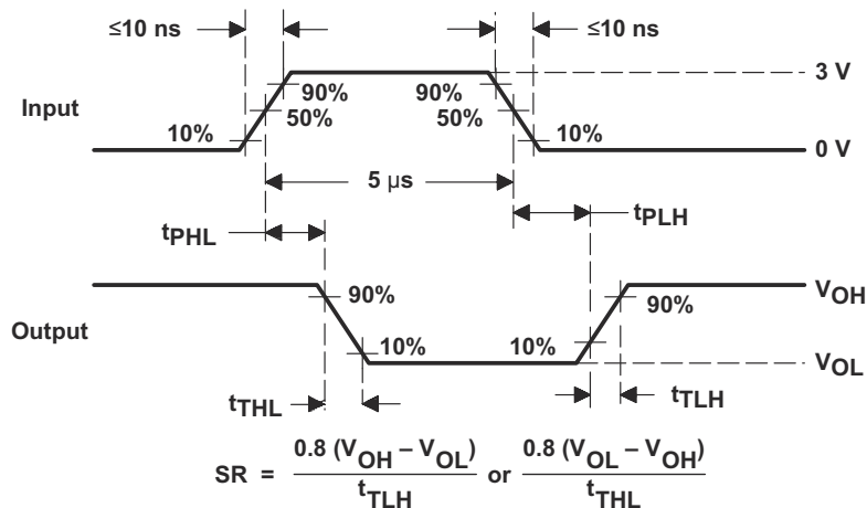
WAVEFORMS
