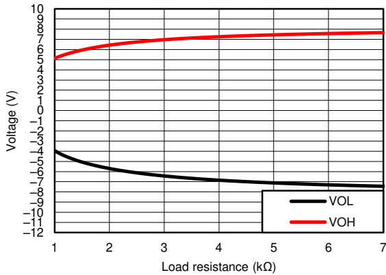
图 8-2. TOUT VOH & VOL vs Load Resistance, Both Drivers Loaded
