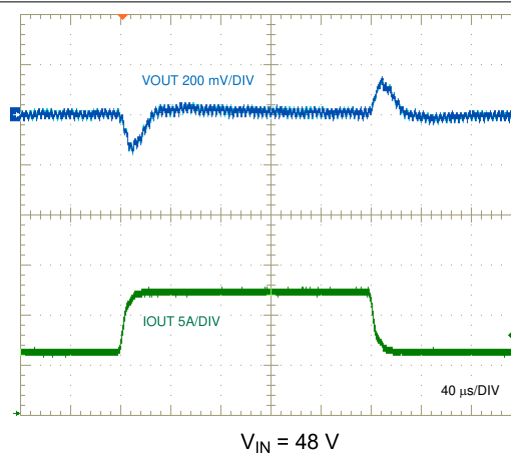
图 9-11. Load Transient Response, 6 A to 12 A to 6 A
