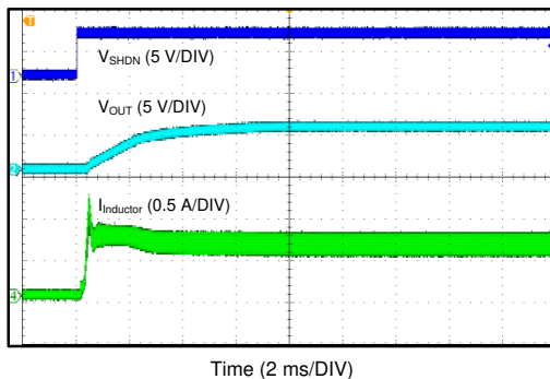
图 8-6. Start-up Waveform
