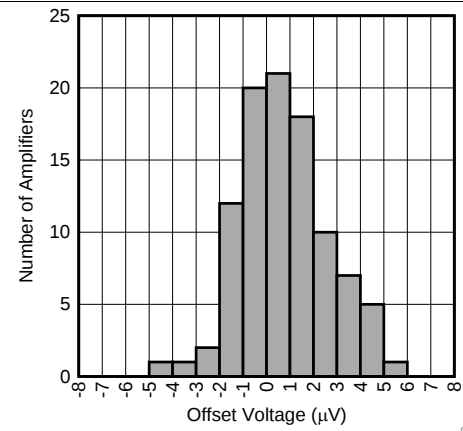
V_S = 3.3\text{V} N = 98 个单元 T_A = 125^\circ\text{C}
