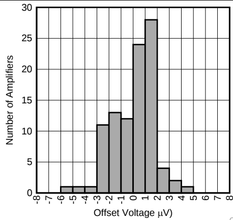
V_S = 1.8\text{V} N = 98 个单元 T_A = -40^\circ\text{C}
