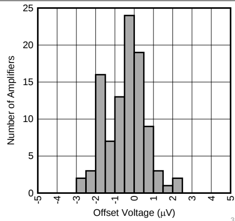
V_S = 3.3\text{V} N = 98 个单元 T_A = 25^\circ\text{C}
