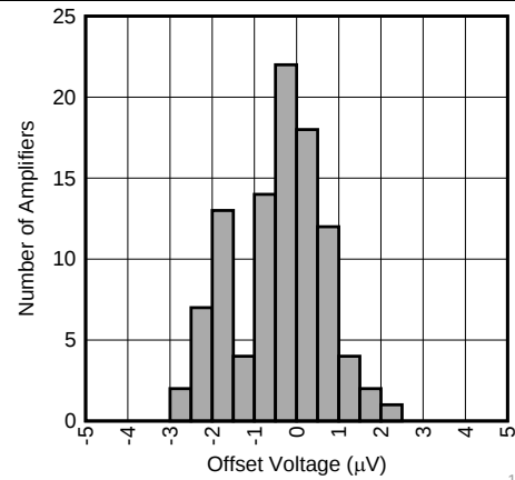
V_S = 1.8\text{V} N = 98 个单元 T_A = 25^\circ\text{C}
