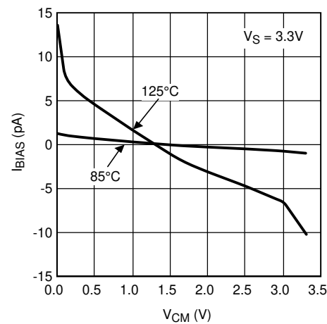
图 5-36. Input Bias Current vs Common Mode Voltage
