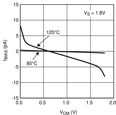
图 5-34. Input Bias Current vs Common Mode Voltage
