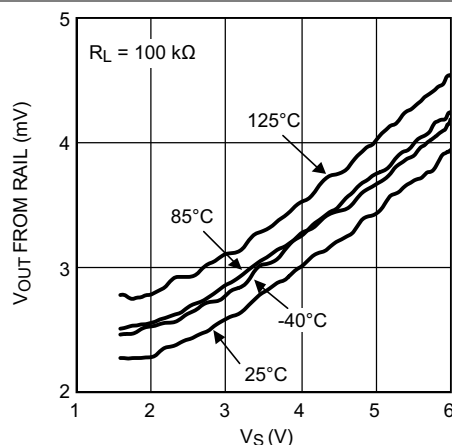
图 5-32. Output Swing Low vs Supply Voltage
