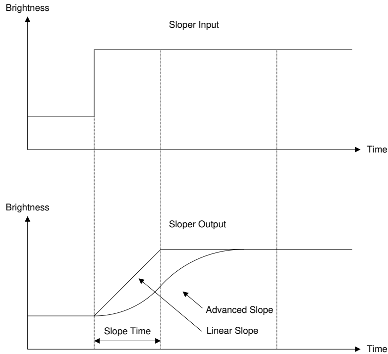
图 6-13. Brightness Sloper
