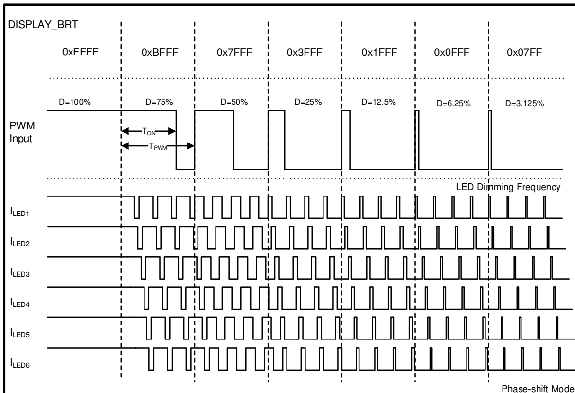
图 6-10. Phase-Shift Dimming Diagram
