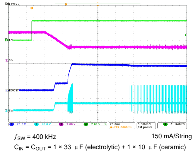
图 7-4. Typical Start-Up
