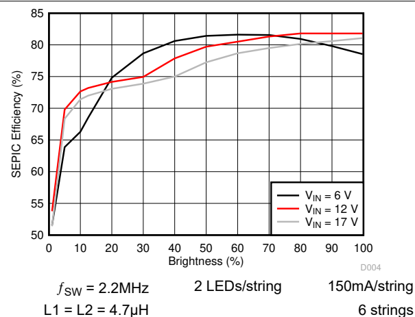
图 5-5. SEPIC Efficiency
