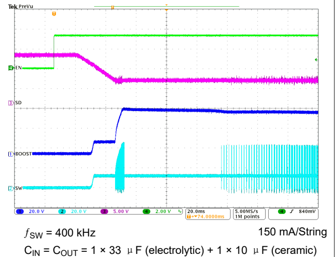
图 8-4. Typical Start-Up
