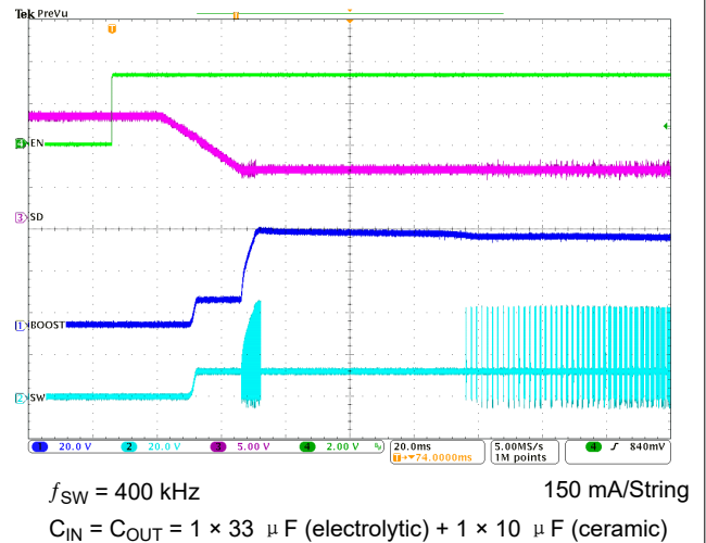
图 7-4. Typical Start-Up
