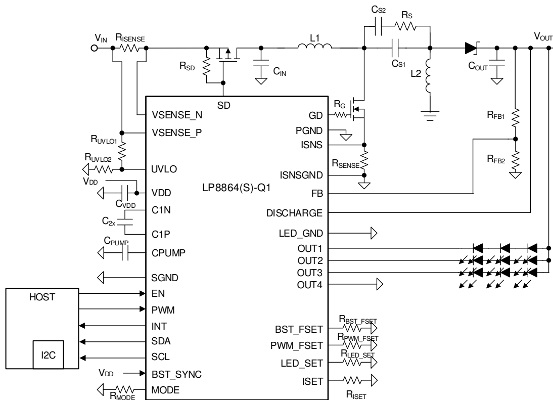
图 7-6. SEPIC 模式 with Three LEDs in Series
