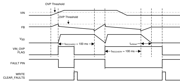
图 6-29. Input OVP Triggering and Recovery
