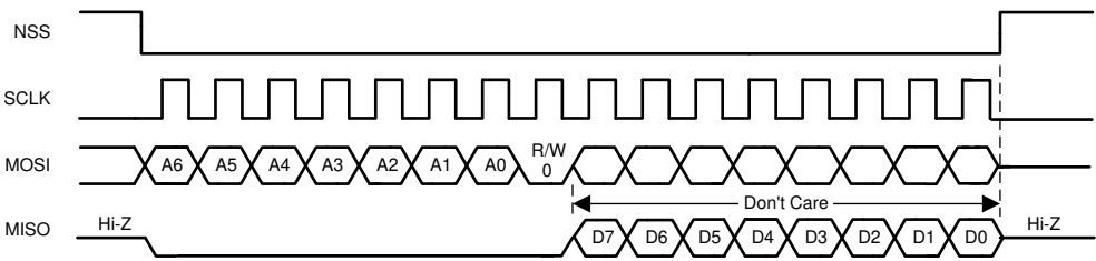
图 6-38. SPI Read Cycle
