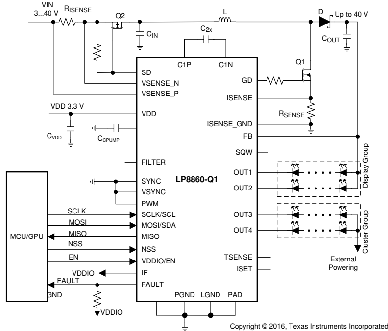
图 7-8. VDD = 3.3V, SPI, 2 Outputs in Display Mode, 2 in Cluster Mode Schematic
