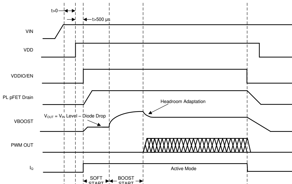
图 6-35. Timing Diagram for the Typical Start-Up and Shutdown
