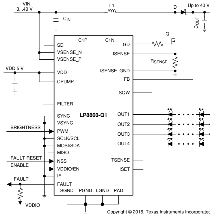
图 7-14. Solution With Minimum External Components
