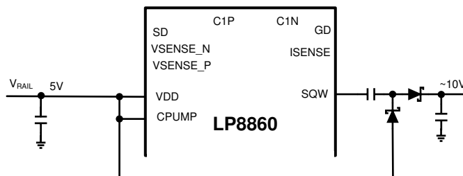
图 6-15. V_{\text{RAIL}} Multiplied by 2
