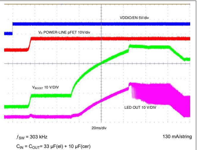
图 7-5. Typical Start-up
