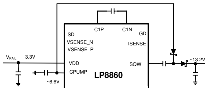
图 6-15. V_{\text{RAIL}} Multiplied by 2
