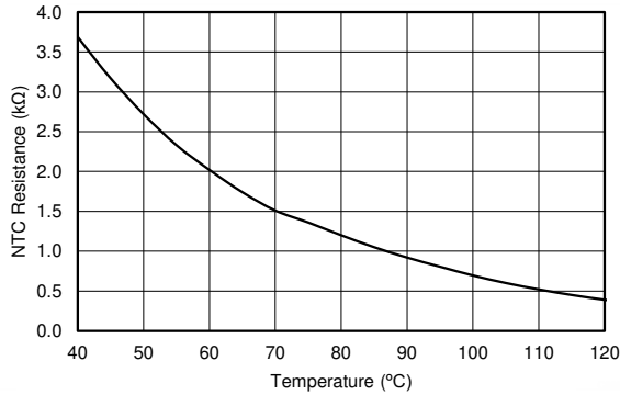
图 7-12. NTC Sensor Resistance vs Temperature
