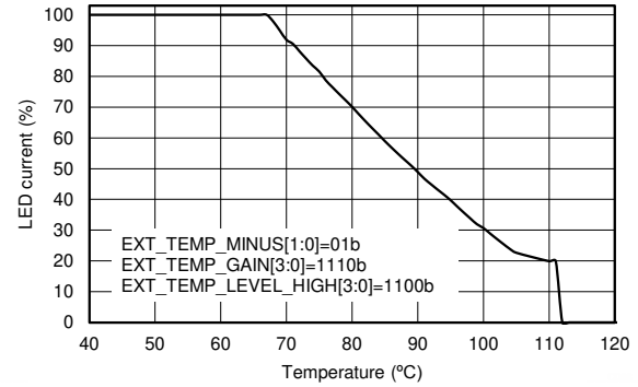
图 7-13. LED Current De-rating vs Temperature
