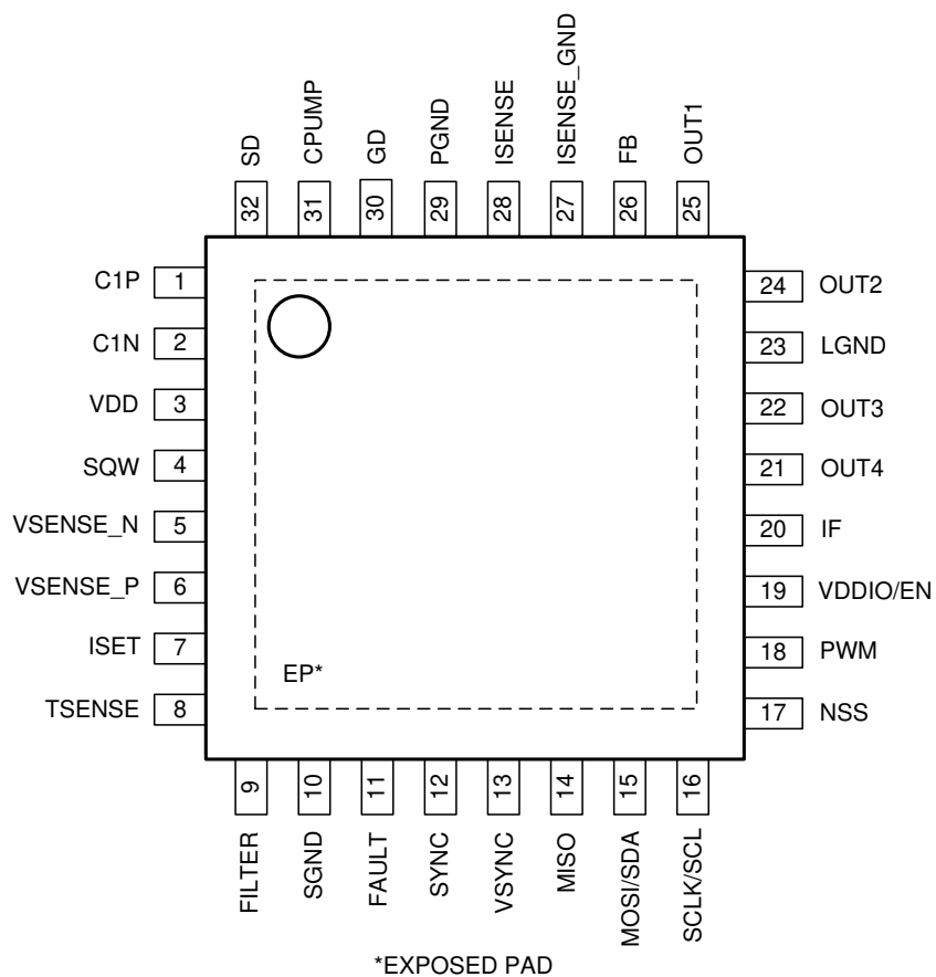
图 4-1. VFP Package 32-Lead PowerPAD™ Quad Flatpack S-PQFP-G32 Top View
