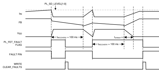
图 6-31. Input OVP Triggering and Recovery
