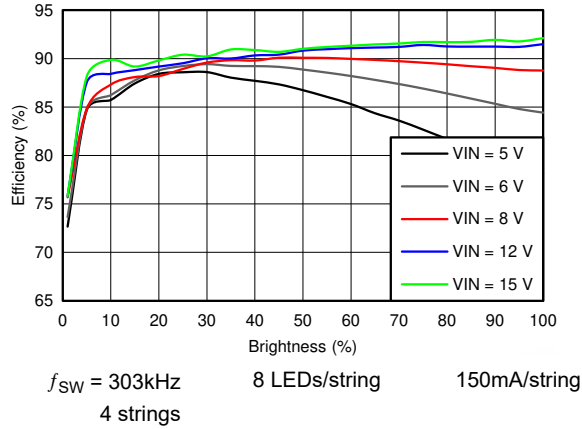
图 5-3. System Efficiency
