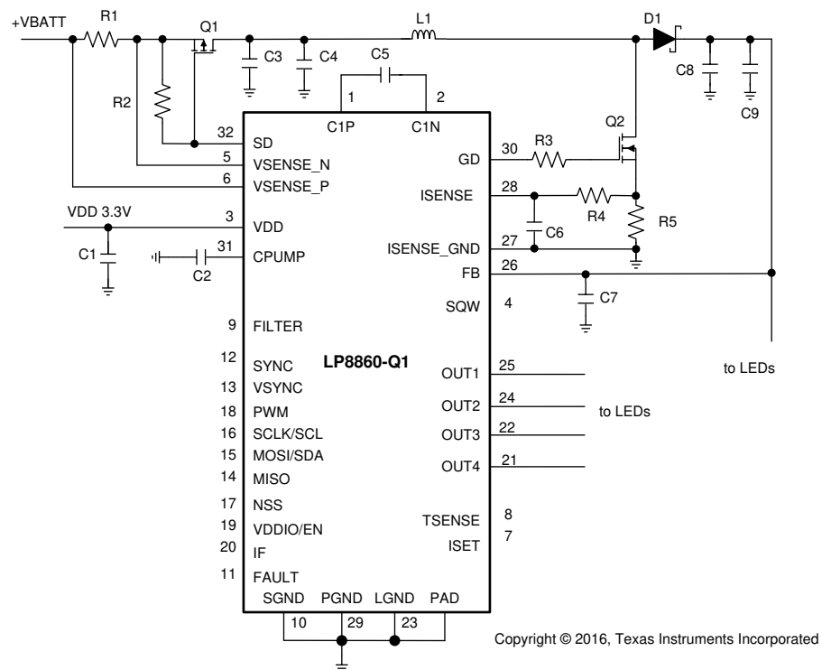
图 7-3. Critical Components for Design
