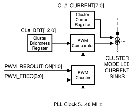
图 6-12. Cluster Mode Block Diagram
