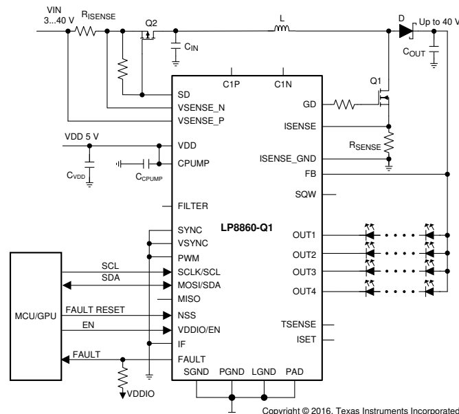
图 7-1. VDD = 5 V, I 2 C, 4 LED Outputs in Display Mode
