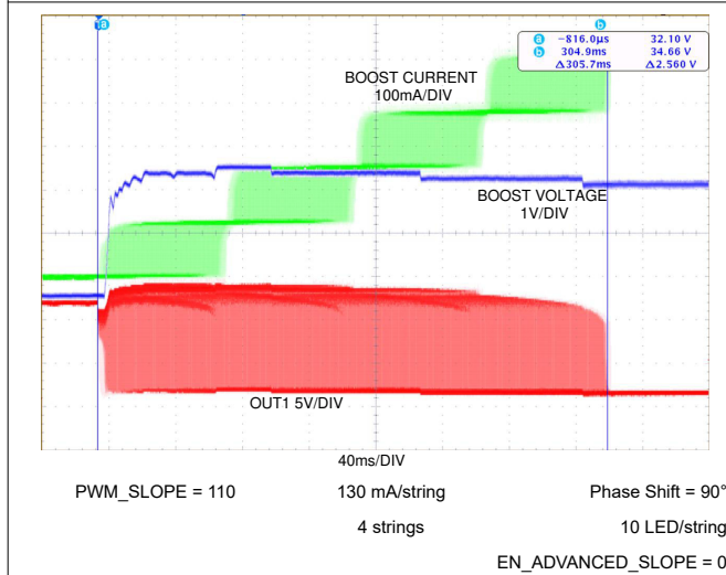
图 7-6. Slope with Phase-Shift Mode
