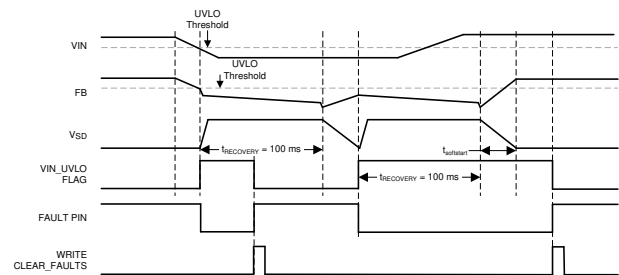
图 6-30. Input UVLO Triggering and Recovery
