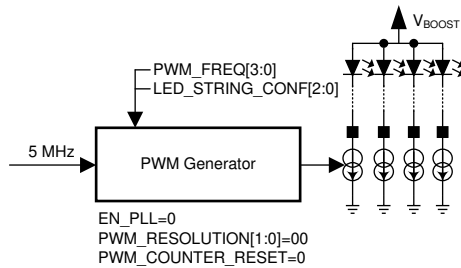
图 6-2. PWM Clocking With Internal Oscillator
