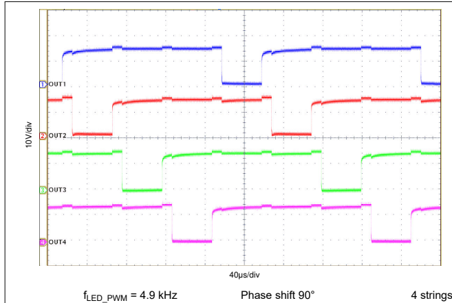
图 7-4. Voltage of LED Outputs Showing Phase-Shift PWM Operation
