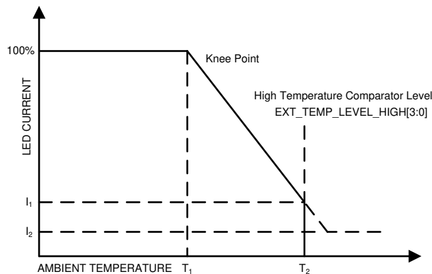
图 6-25. Current Dimming for High Ambient Temperature
