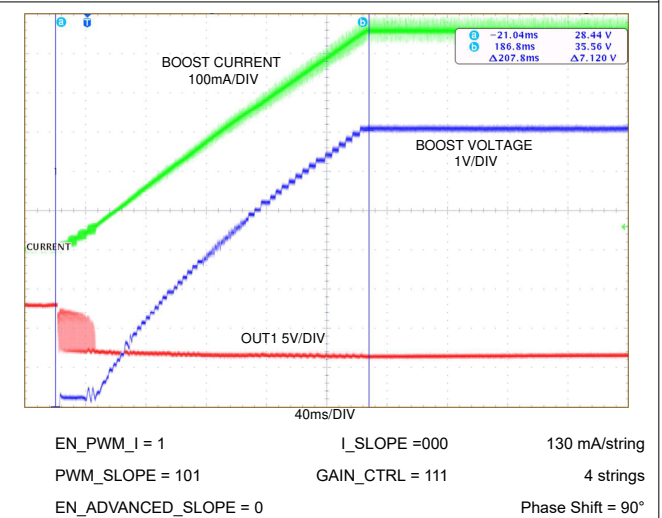
图 7-7. Slope With Hybrid Dimming and Phase Shift
