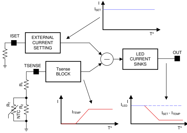
图 6-27. Temperature-Dependent NTC Current (Subtracted from ISET Current)
