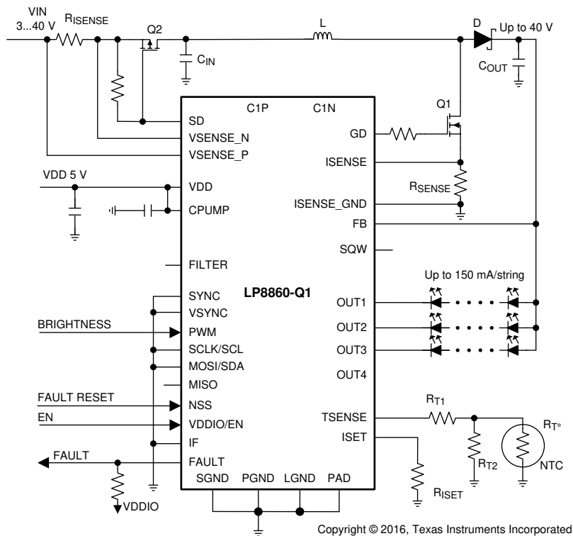
图 7-11. Three-Channel Configuration without Serial Interface
