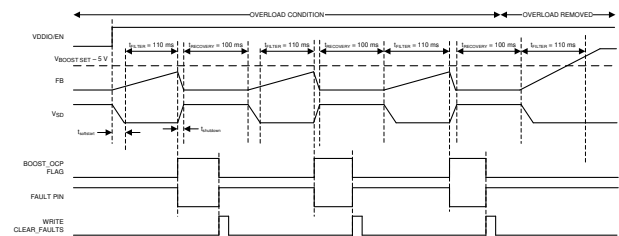
图 6-32. Boost OCP Triggering and Recovery
