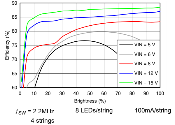
图 5-4. System Efficiency
