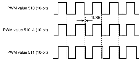
图 6-5. Example of the Dithering, 1-Bit Dither, 10-Bit Resolution
