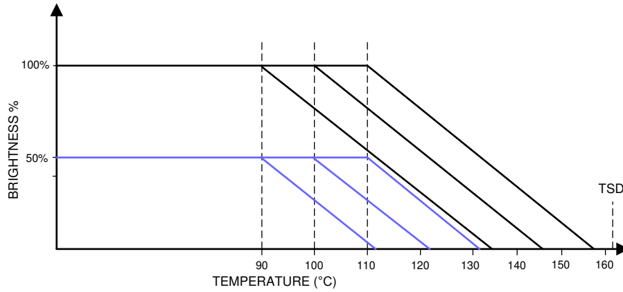
图 6-22. Thermal De-Rating Function Example With 100% and 50% Brightness
