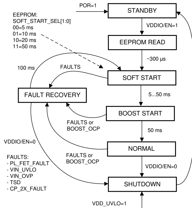
图 6-34. State Diagram
