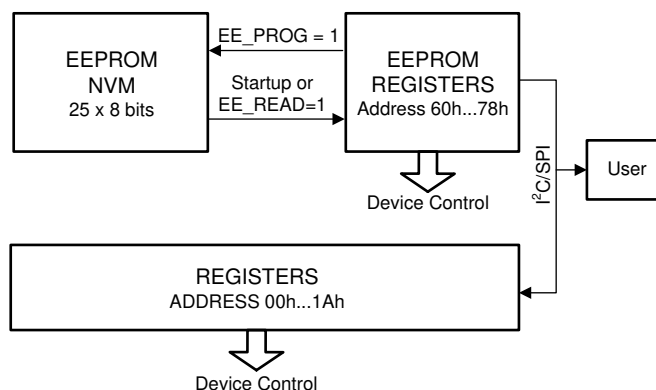
图 6-36. EEPROM and Register Configuration
