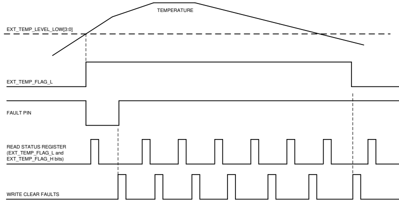
图 6-24. Timing Diagram for LED Current Limitation With NTC
