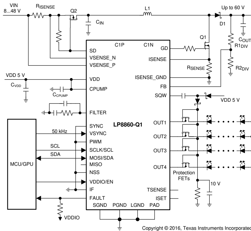
图 7-9. VDD = 5 V, I 2 C, High-Voltage Output with Output Protection FETs Circuits
