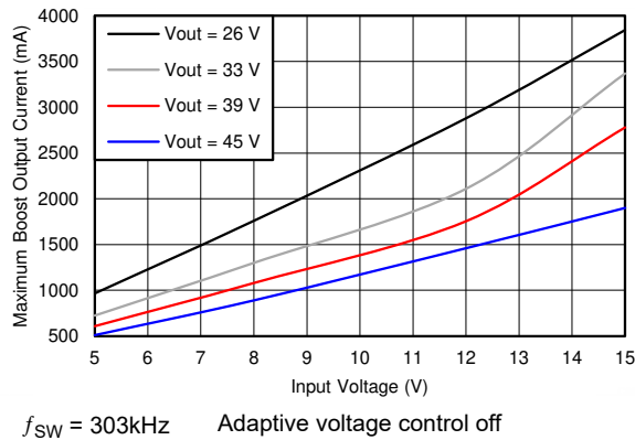
图 5-5. Boost Maximum Output Current
