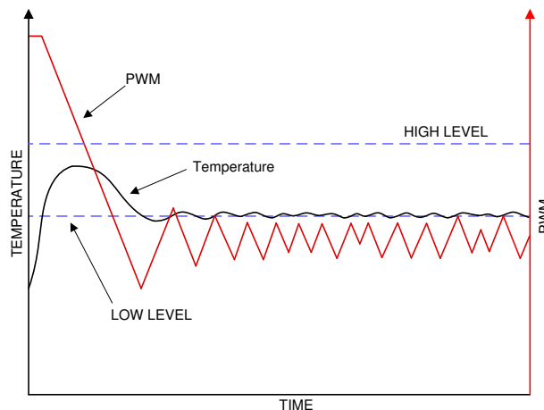
图 6-23. LED Current Limitation With NTC
