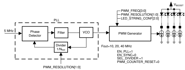
图 6-3. PWM Clocking With PLL, Internal Oscillator as Reference
