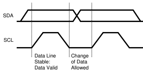
图 6-39. Bit Transfer
