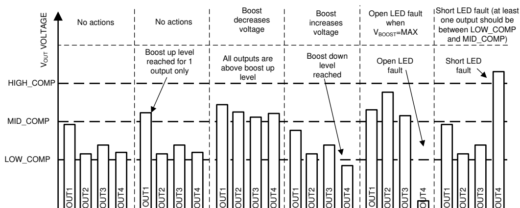
图 6-21. Protection and Boost Adaptation Algorithms
