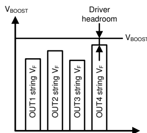
图 6-19. Boost Voltage Adaptation
