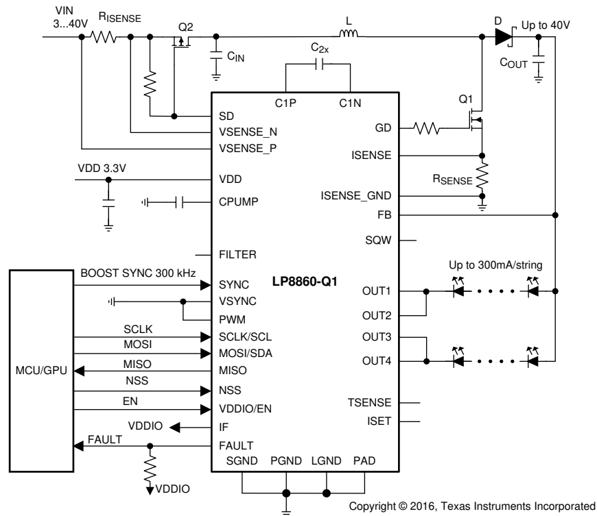
图 7-10. Two Channels at 300 mA/String, VDD = 3.3 V, SPI
