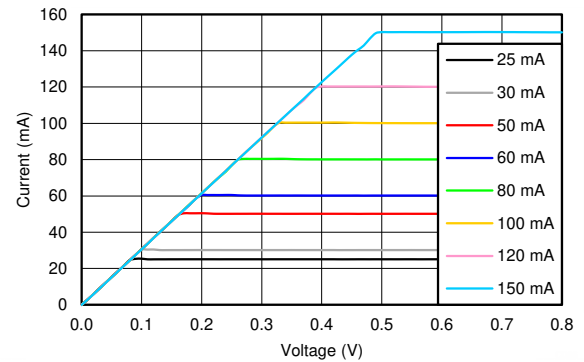
图 5-6. LED Current vs Headroom Voltage
