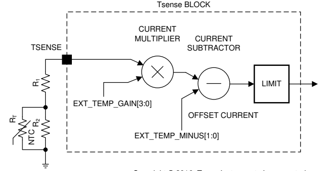
图 6-28. NTC Current Processing — Scaling, Shift, and Limitation
