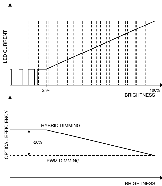
图 6-8. Optical Efficiency Improvement With PWM and Current Dimming
