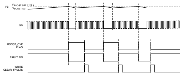
图 6-33. Boost OVP Triggering and Recovery
