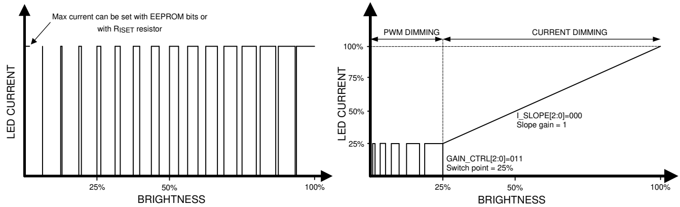
图 6-7. Principles of PWM Dimming and Hybrid PWM and Current Dimming
