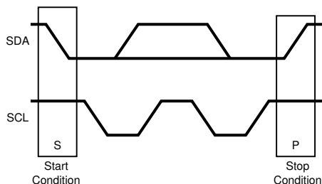
图 6-41. Stop and Start Conditions
