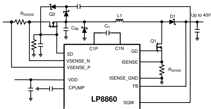
图 6-16. V_{\text{RAIL}} Multiplied by 4
